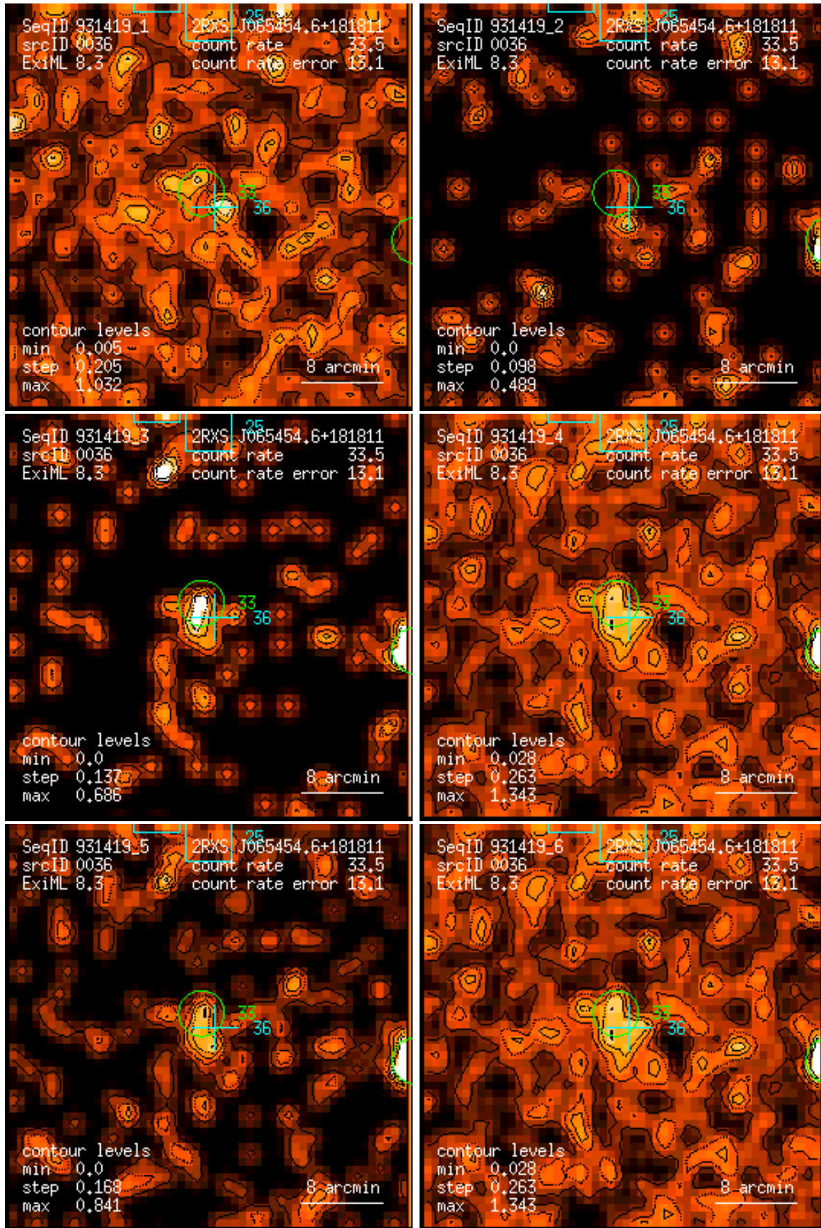
Figure 36: RASS 931419: detection 0036: band rate images, Gaussian filter: (1) PSPC channels 11 – 41, (2) 52 – 90, (3) 91 – 201, (4) 11 – 235, (5) 52 – 201, (6) 11 – 201. Broad band rates in counts/ks. Band rate contour levels in counts/ks/arcmin 2 .
