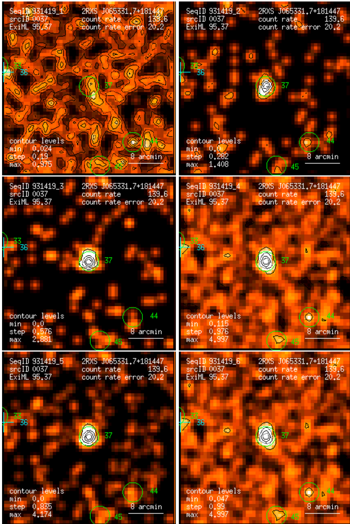
Figure 37: RASS 931419: detection 0037: band rate images, Gaussian filter: (1) PSPC channels 11 – 41, (2) 52 – 90, (3) 91 – 201, (4) 11 – 235, (5) 52 – 201, (6) 11 – 201. Broad band rates in counts/ks. Band rate contour levels in counts/ks/arcmin 2 .
