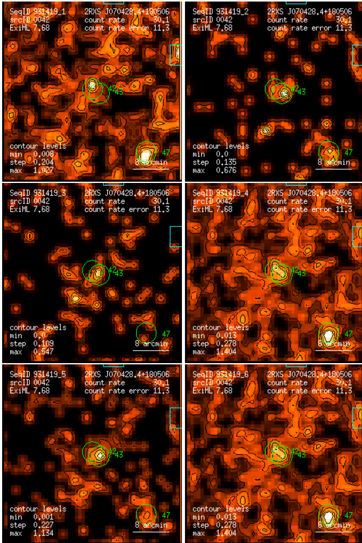
Figure 42: RASS 931419: detection 0042: band rate images, Gaussian filter: (1) PSPC channels 11 – 41, (2) 52 – 90, (3) 91 – 201, (4) 11 – 235, (5) 52 – 201, (6) 11 – 201. Broad band rates in counts/ks. Band rate contour levels in counts/ks/arcmin 2 .
