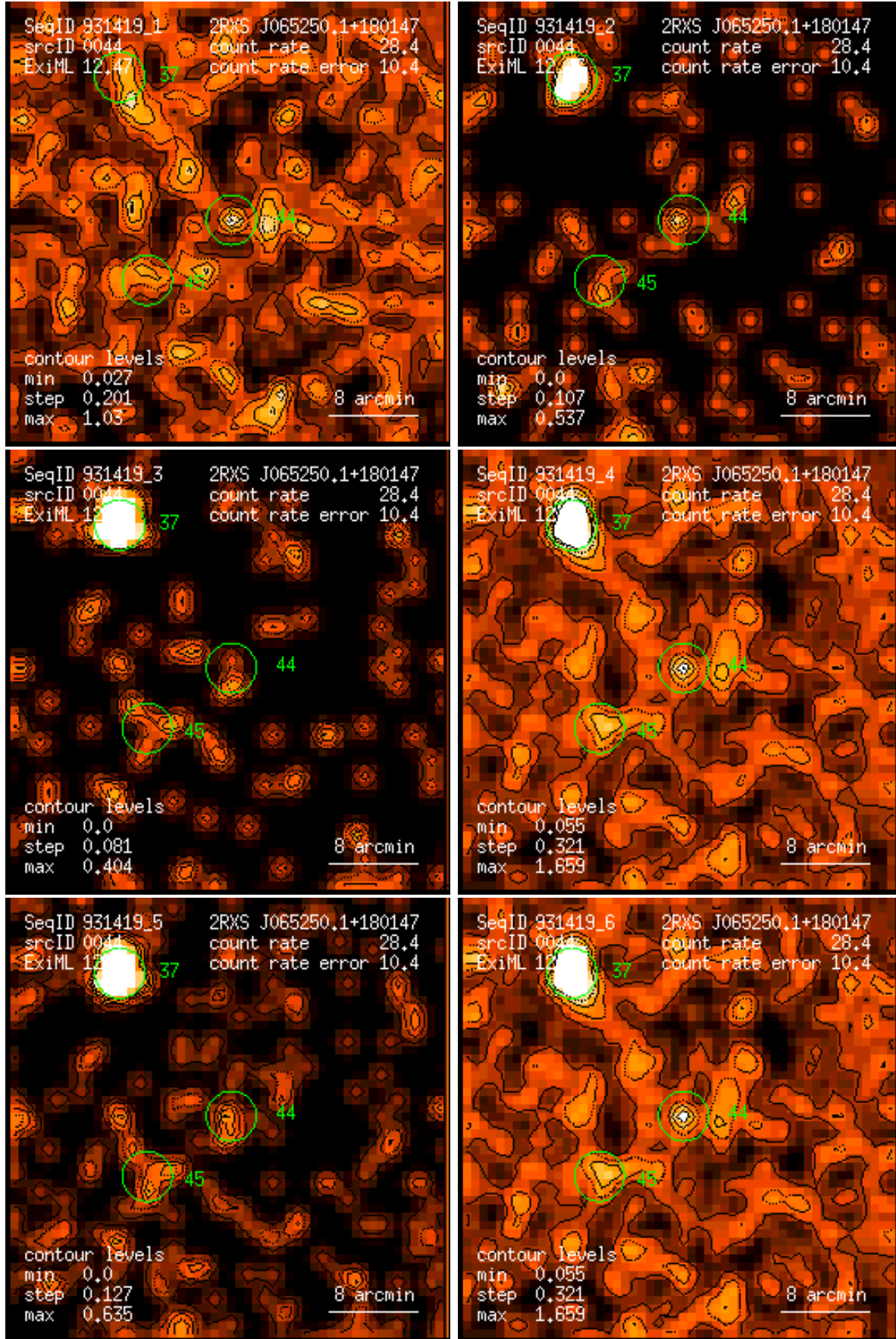
Figure 44: RASS 931419: detection 0044: band rate images, Gaussian filter: (1) PSPC channels 11 – 41, (2) 52 – 90, (3) 91 – 201, (4) 11 – 235, (5) 52 – 201, (6) 11 – 201. Broad band rates in counts/ks. Band rate contour levels in counts/ks/arcmin 2 .
