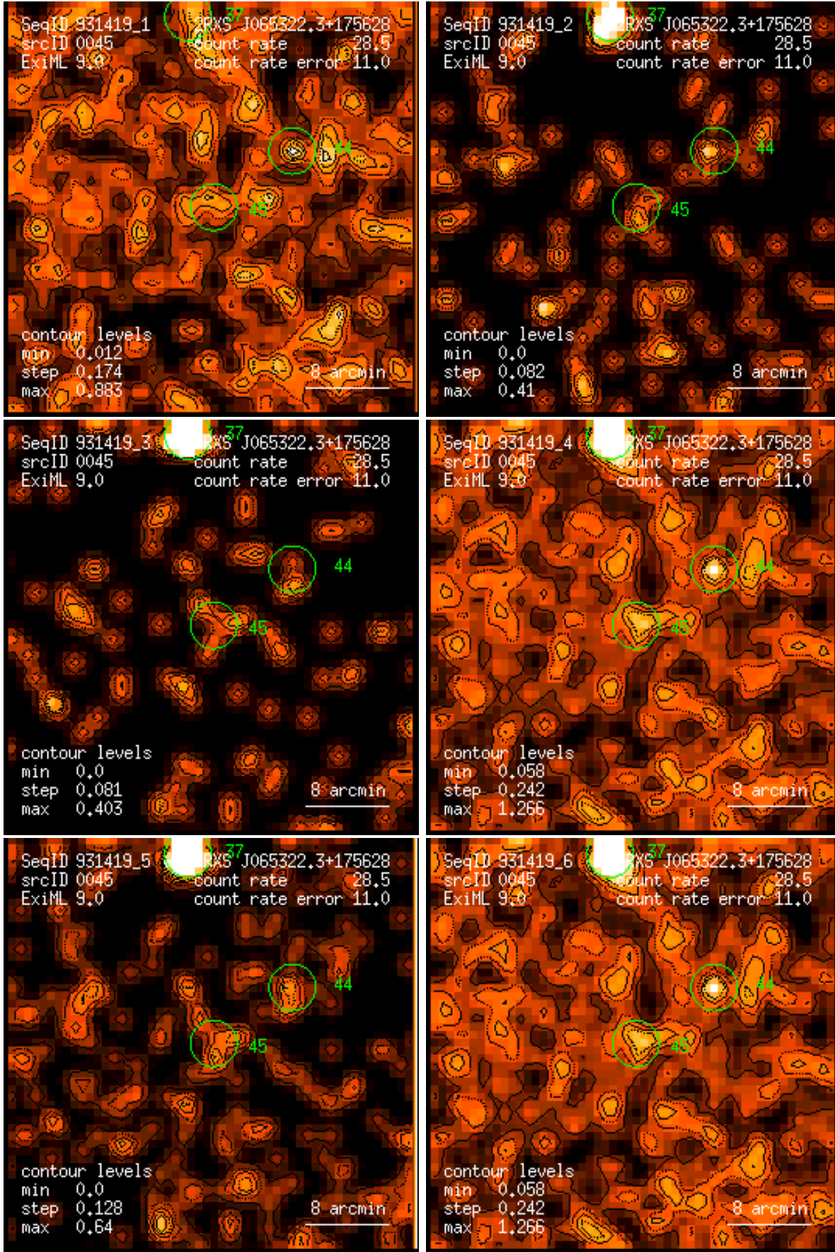
Figure 45: RASS 931419: detection 0045: band rate images, Gaussian filter: (1) PSPC channels 11 – 41, (2) 52 – 90, (3) 91 – 201, (4) 11 – 235, (5) 52 – 201, (6) 11 – 201. Broad band rates in counts/ks. Band rate contour levels in counts/ks/arcmin 2 .
