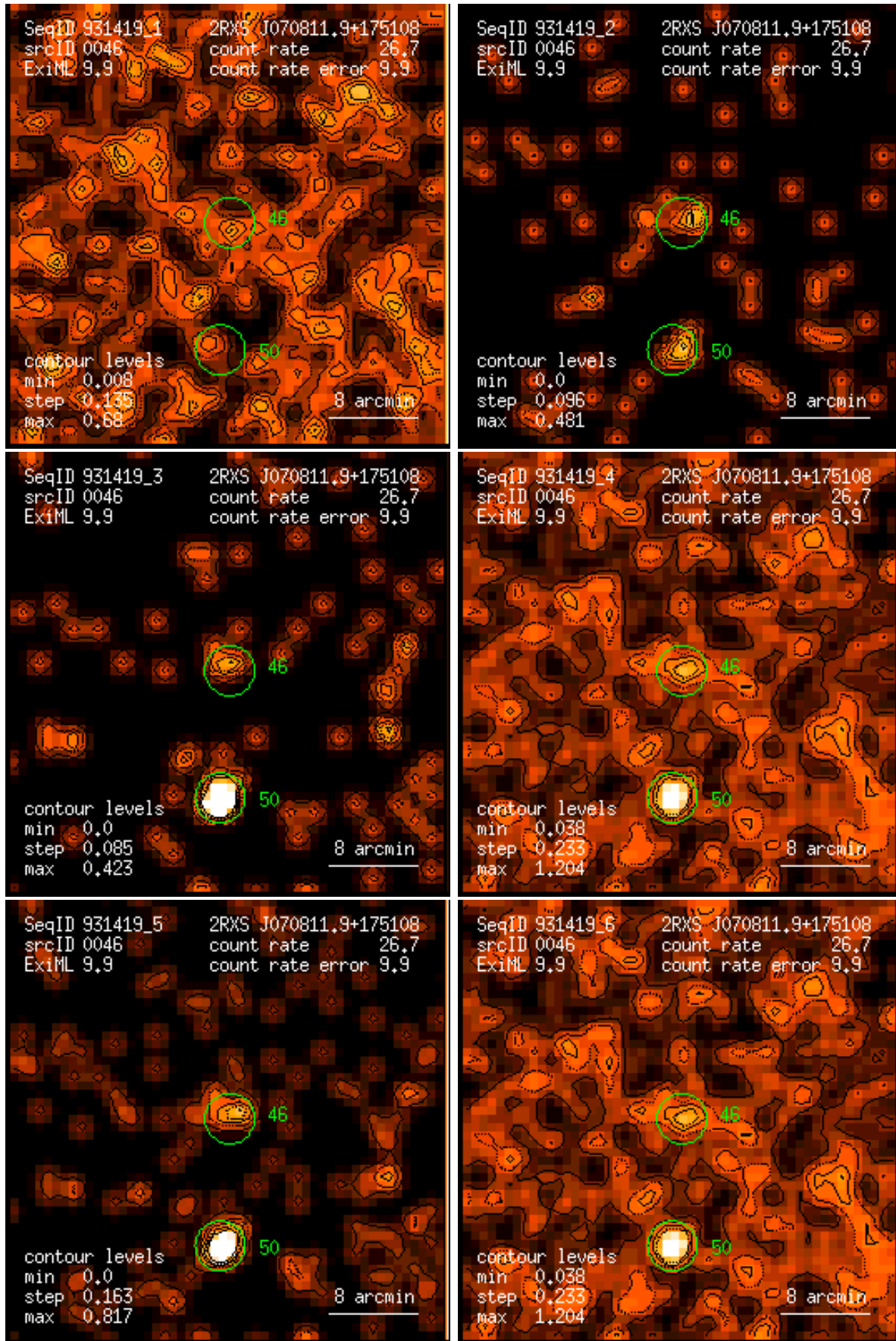
Figure 46: RASS 931419: detection 0046: band rate images, Gaussian filter: (1) PSPC channels 11 – 41, (2) 52 – 90, (3) 91 – 201, (4) 11 – 235, (5) 52 – 201, (6) 11 – 201. Broad band rates in counts/ks. Band rate contour levels in counts/ks/arcmin 2 .
