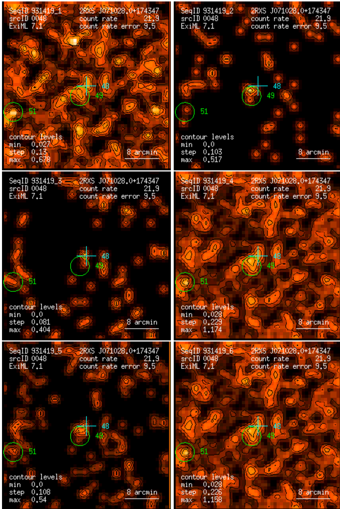
Figure 48: RASS 931419: detection 0048: band rate images, Gaussian filter: (1) PSPC channels 11 – 41, (2) 52 – 90, (3) 91 – 201, (4) 11 – 235, (5) 52 – 201, (6) 11 – 201. Broad band rates in counts/ks. Band rate contour levels in counts/ks/arcmin 2 .
