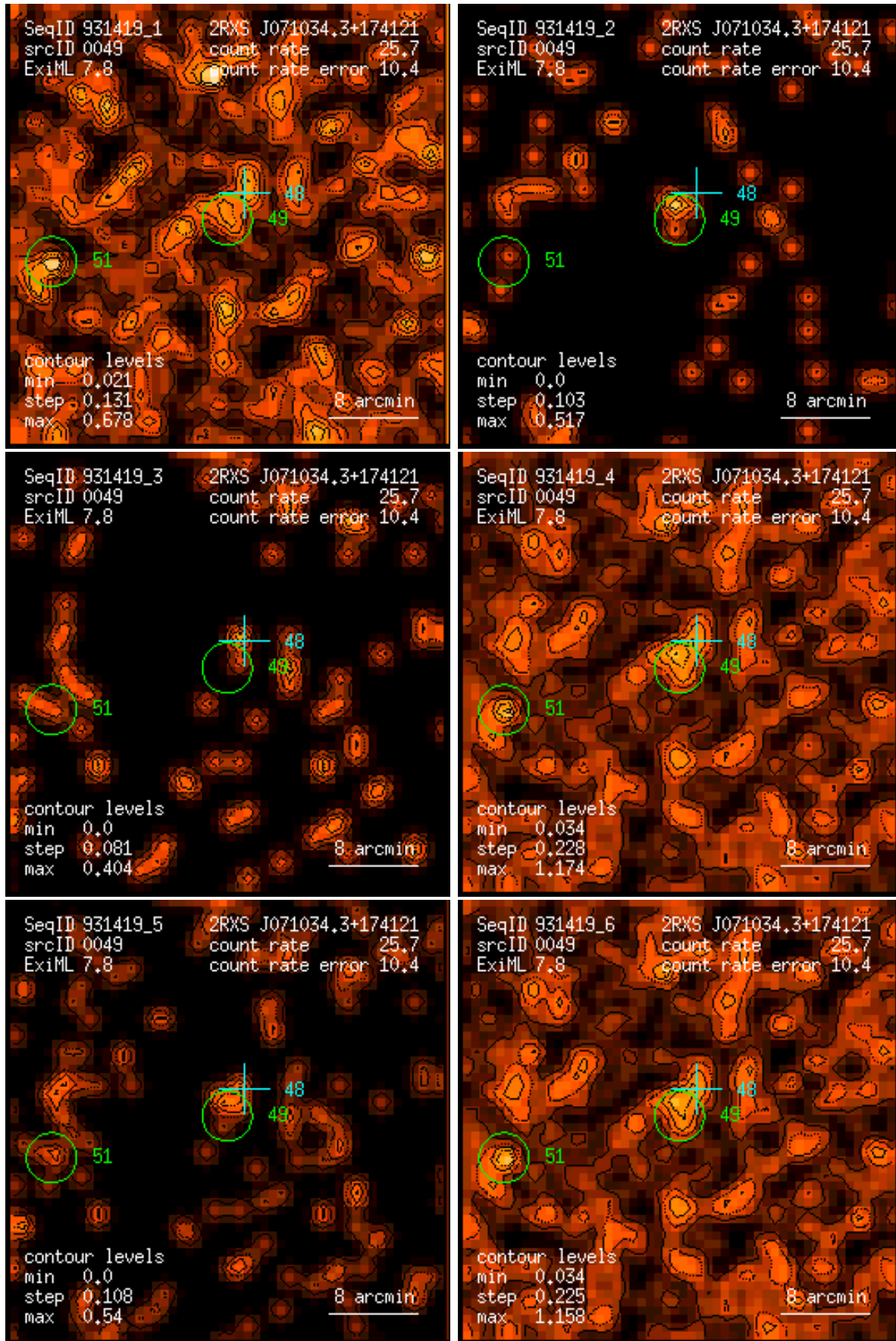
Figure 49: RASS 931419: detection 0049: band rate images, Gaussian filter: (1) PSPC channels 11 – 41, (2) 52 – 90, (3) 91 – 201, (4) 11 – 235, (5) 52 – 201, (6) 11 – 201. Broad band rates in counts/ks. Band rate contour levels in counts/ks/arcmin 2 .
