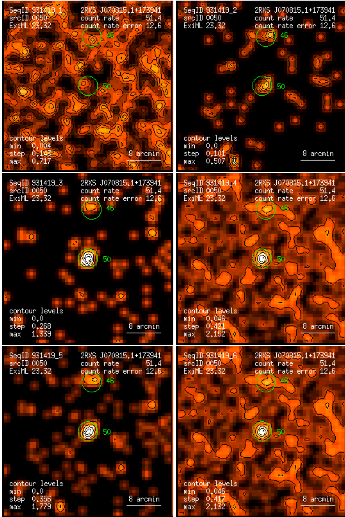
Figure 50: RASS 931419: detection 0050: band rate images, Gaussian filter: (1) PSPC channels 11 – 41, (2) 52 – 90, (3) 91 – 201, (4) 11 – 235, (5) 52 – 201, (6) 11 – 201. Broad band rates in counts/ks. Band rate contour levels in counts/ks/arcmin 2 .
