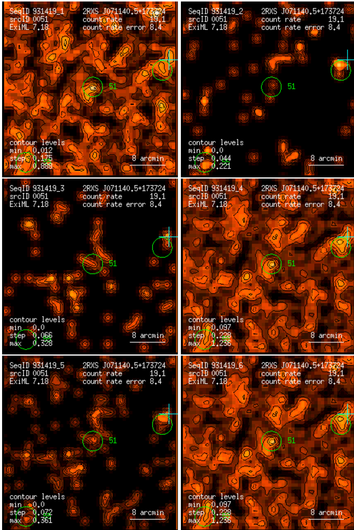
Figure 51: RASS 931419: detection 0051: band rate images, Gaussian filter: (1) PSPC channels 11 – 41, (2) 52 – 90, (3) 91 – 201, (4) 11 – 235, (5) 52 – 201, (6) 11 – 201. Broad band rates in counts/ks. Band rate contour levels in counts/ks/arcmin 2 .
