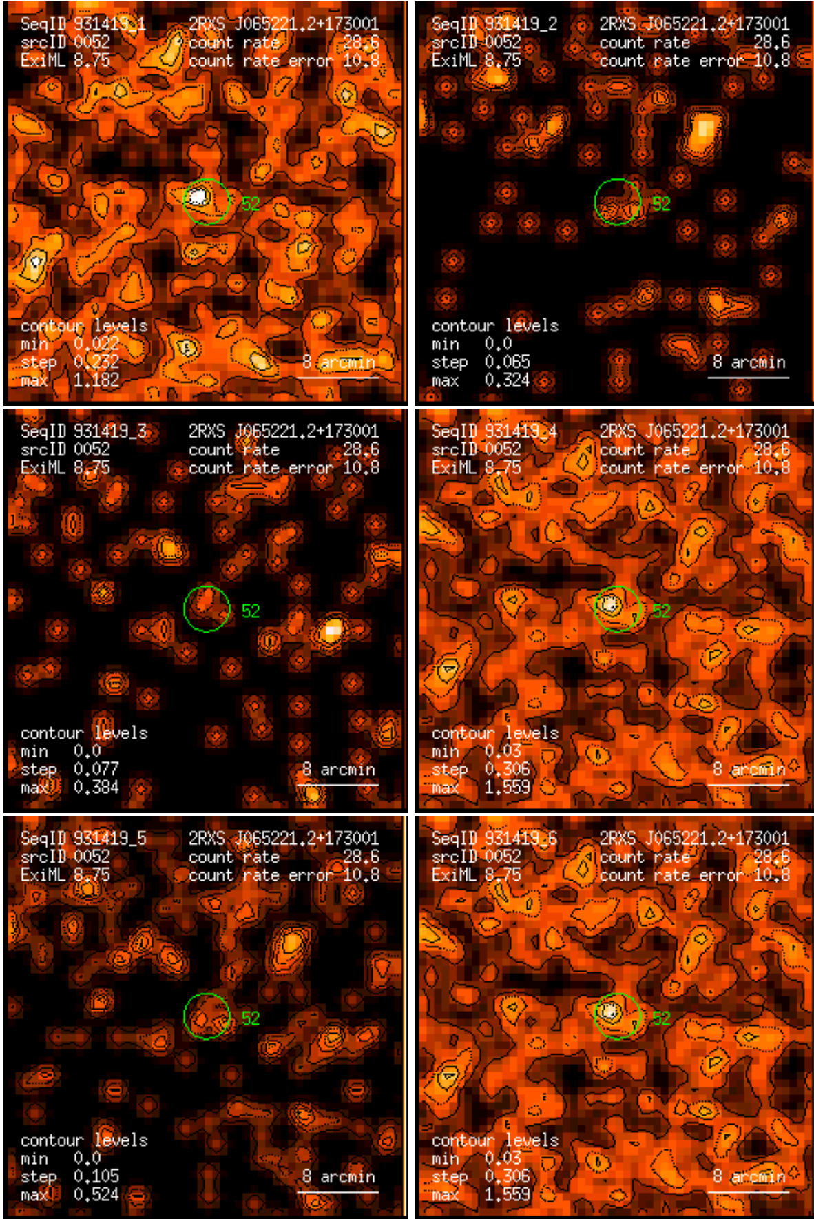
Figure 52: RASS 931419: detection 0052: band rate images, Gaussian filter: (1) PSPC channels 11 – 41, (2) 52 – 90, (3) 91 – 201, (4) 11 – 235, (5) 52 – 201, (6) 11 – 201. Broad band rates in counts/ks. Band rate contour levels in counts/ks/arcmin 2 .
