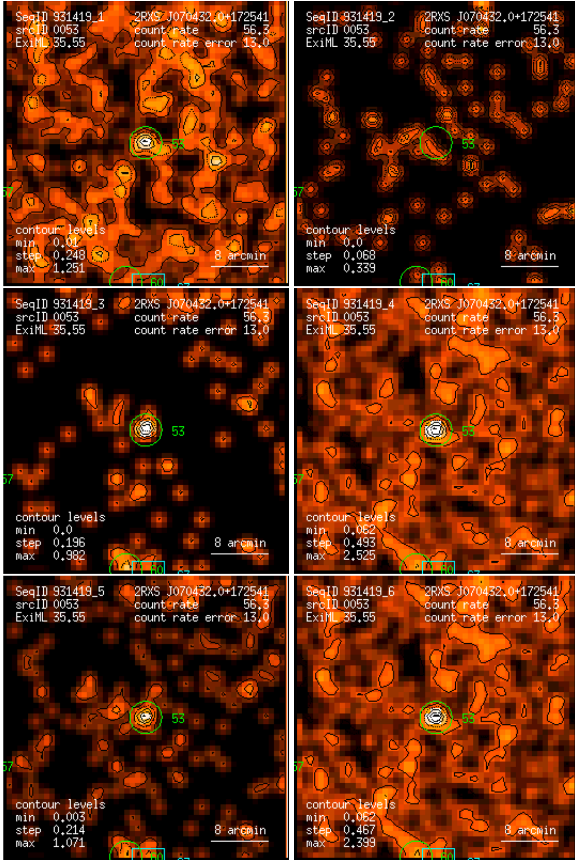
Figure 53: RASS 931419: detection 0053: band rate images, Gaussian filter: (1) PSPC channels 11 – 41, (2) 52 – 90, (3) 91 – 201, (4) 11 – 235, (5) 52 – 201, (6) 11 – 201. Broad band rates in counts/ks. Band rate contour levels in counts/ks/arcmin 2 .
