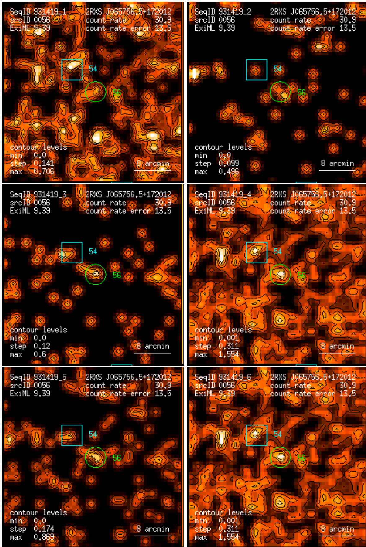
Figure 56: RASS 931419: detection 0056: band rate images, Gaussian filter: (1) PSPC channels 11 – 41, (2) 52 – 90, (3) 91 – 201, (4) 11 – 235, (5) 52 – 201, (6) 11 – 201. Broad band rates in counts/ks. Band rate contour levels in counts/ks/arcmin 2 .
