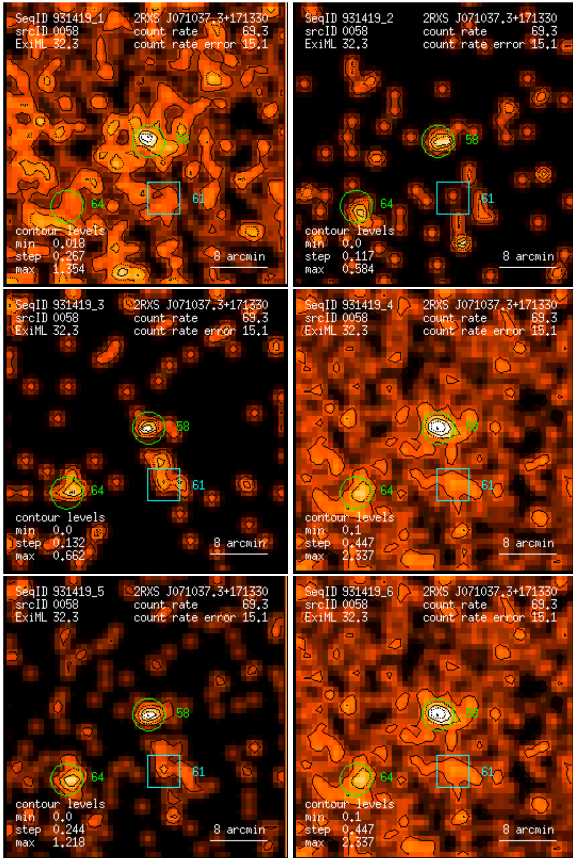
Figure 58: RASS 931419: detection 0058: band rate images, Gaussian filter: (1) PSPC channels 11 – 41, (2) 52 – 90, (3) 91 – 201, (4) 11 – 235, (5) 52 – 201, (6) 11 – 201. Broad band rates in counts/ks. Band rate contour levels in counts/ks/arcmin 2 .
