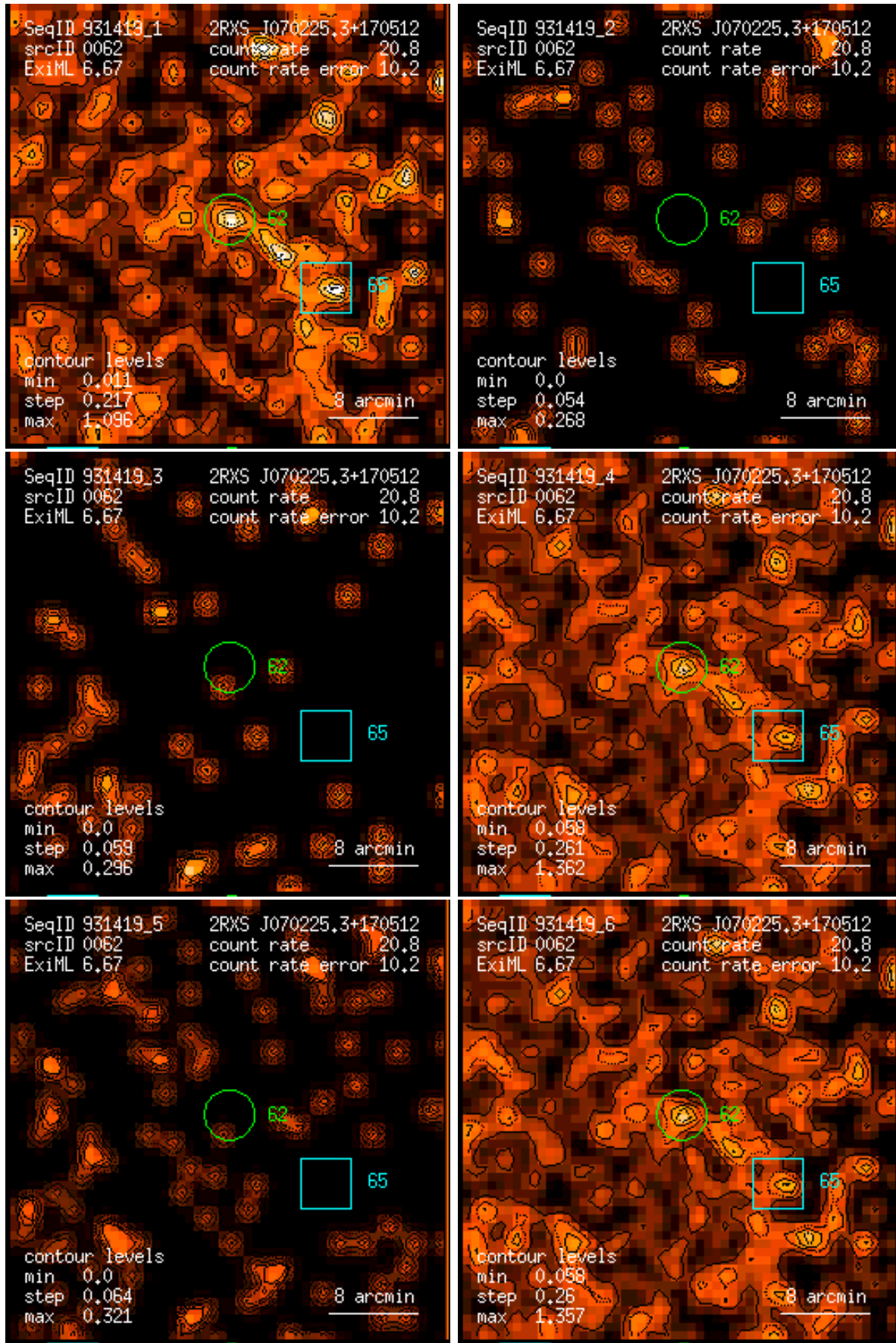
Figure 62: RASS 931419: detection 0062: band rate images, Gaussian filter: (1) PSPC channels 11 – 41, (2) 52 – 90, (3) 91 – 201, (4) 11 – 235, (5) 52 – 201, (6) 11 – 201. Broad band rates in counts/ks. Band rate contour levels in counts/ks/arcmin 2 .
