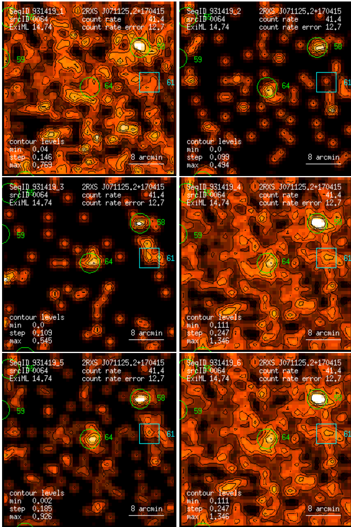
Figure 64: RASS 931419: detection 0064: band rate images, Gaussian filter: (1) PSPC channels 11 – 41, (2) 52 – 90, (3) 91 – 201, (4) 11 – 235, (5) 52 – 201, (6) 11 – 201. Broad band rates in counts/ks. Band rate contour levels in counts/ks/arcmin 2 .
