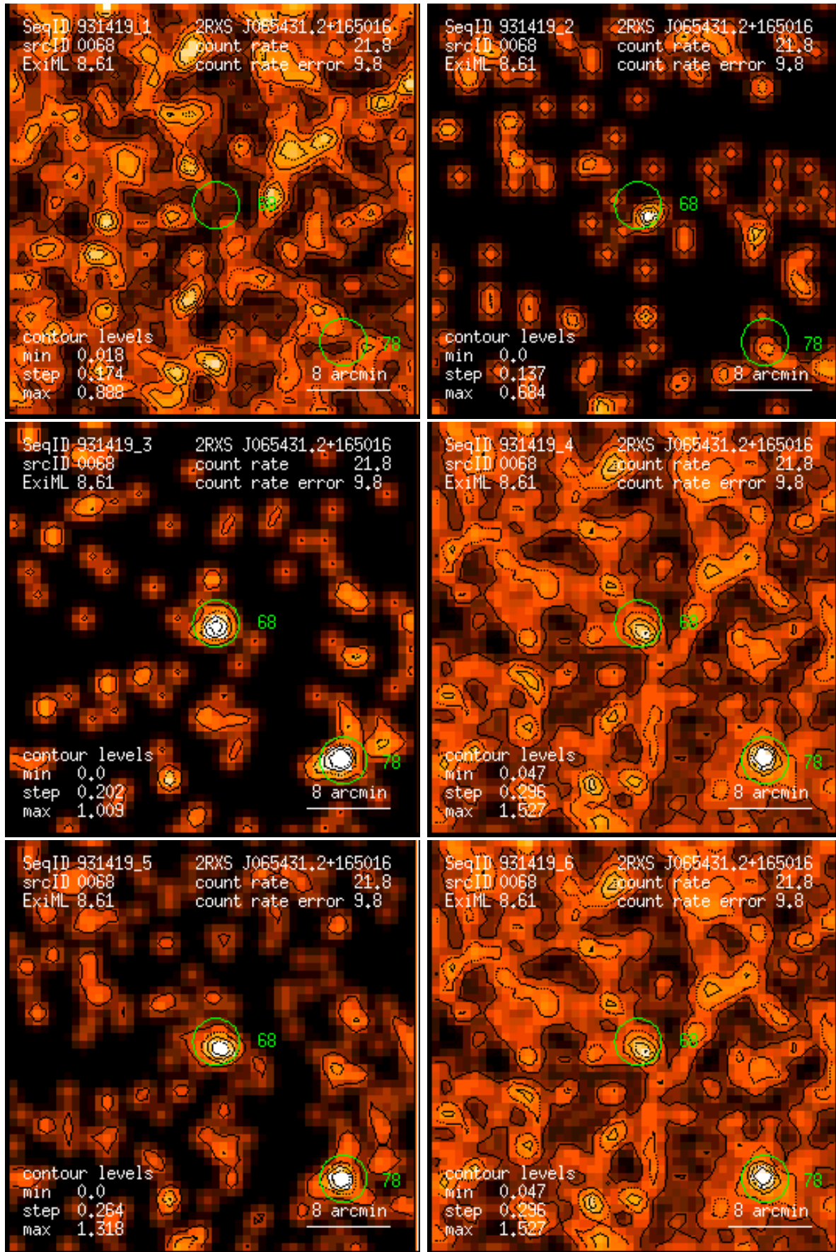
Figure 68: RASS 931419: detection 0068: band rate images, Gaussian filter: (1) PSPC channels 11 – 41, (2) 52 – 90, (3) 91 – 201, (4) 11 – 235, (5) 52 – 201, (6) 11 – 201. Broad band rates in counts/ks. Band rate contour levels in counts/ks/arcmin 2 .
