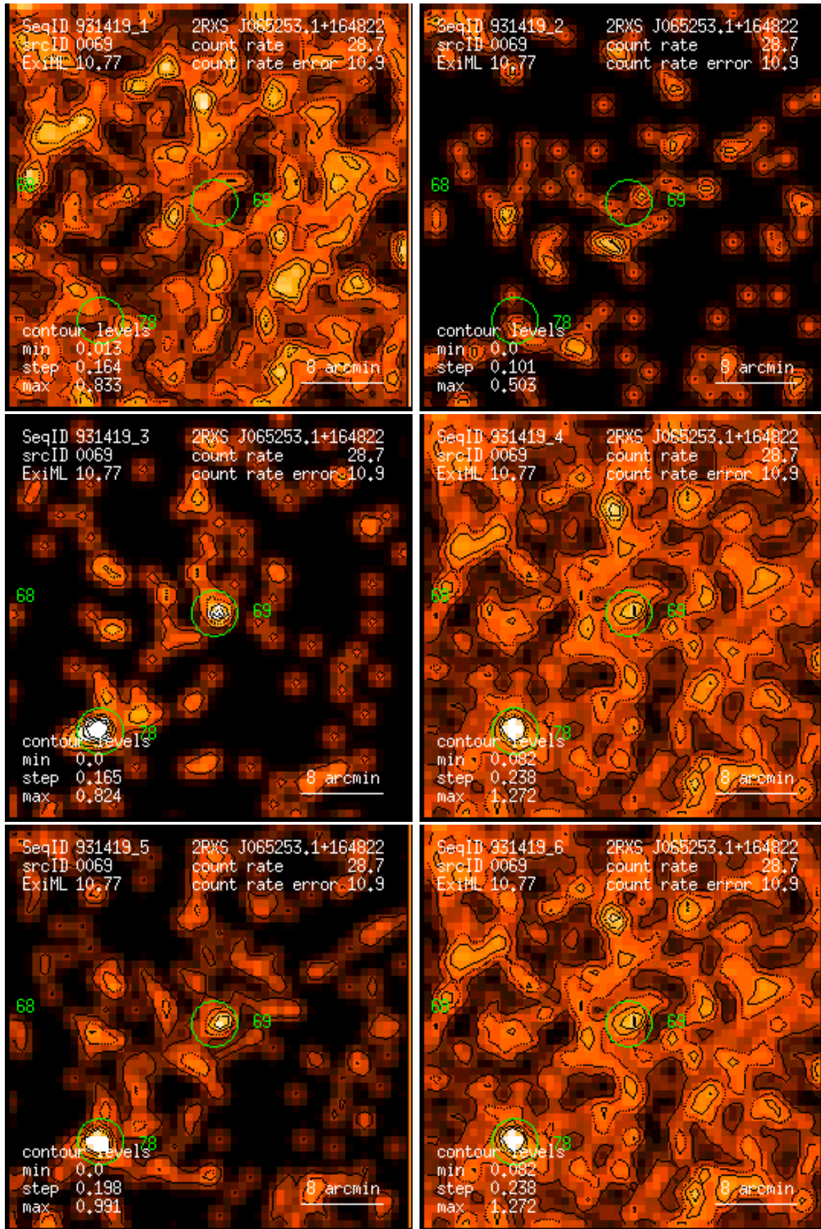
Figure 69: RASS 931419: detection 0069: band rate images, Gaussian filter: (1) PSPC channels 11 – 41, (2) 52 – 90, (3) 91 – 201, (4) 11 – 235, (5) 52 – 201, (6) 11 – 201. Broad band rates in counts/ks. Band rate contour levels in counts/ks/arcmin 2 .
