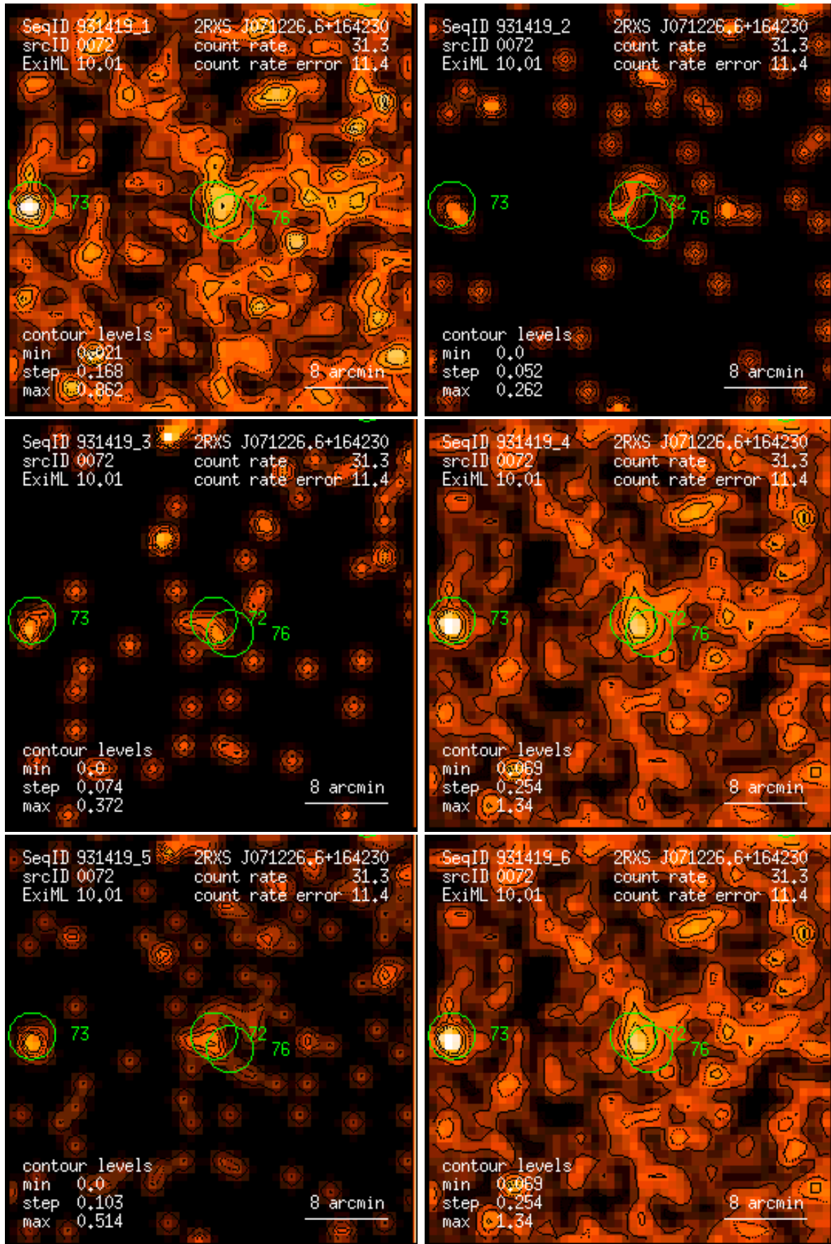
Figure 72: RASS 931419: detection 0072: band rate images, Gaussian filter: (1) PSPC channels 11 – 41, (2) 52 – 90, (3) 91 – 201, (4) 11 – 235, (5) 52 – 201, (6) 11 – 201. Broad band rates in counts/ks. Band rate contour levels in counts/ks/arcmin 2 .
