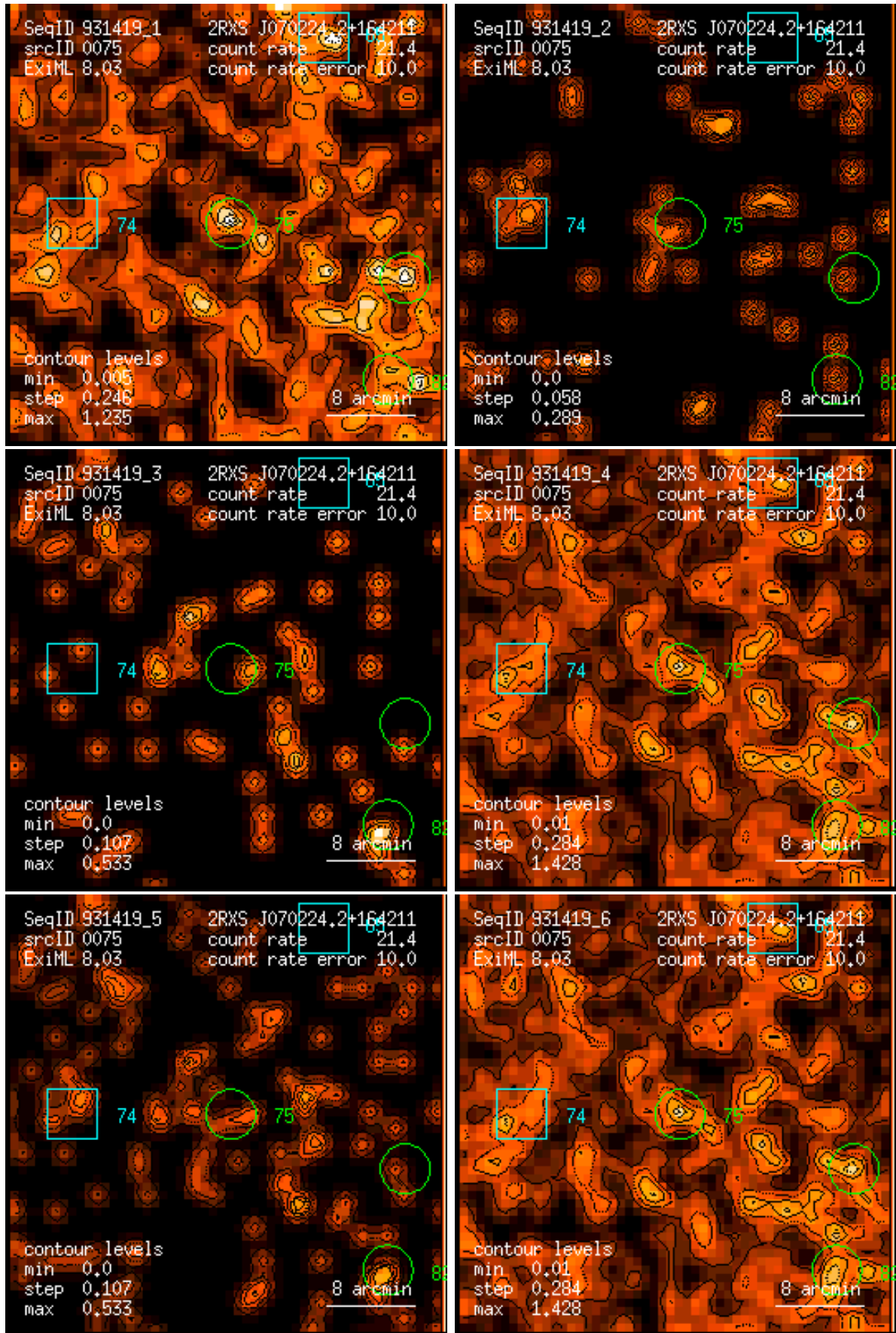
Figure 75: RASS 931419: detection 0075: band rate images, Gaussian filter: (1) PSPP channels 11 – 41, (2) 52 – 90, (3) 91 – 201, (4) 11 – 235, (5) 52 – 201, (6) 11 – 201. Broad band rates in counts/ks. Band rate contour levels in counts/ks/arcmin 2 .
