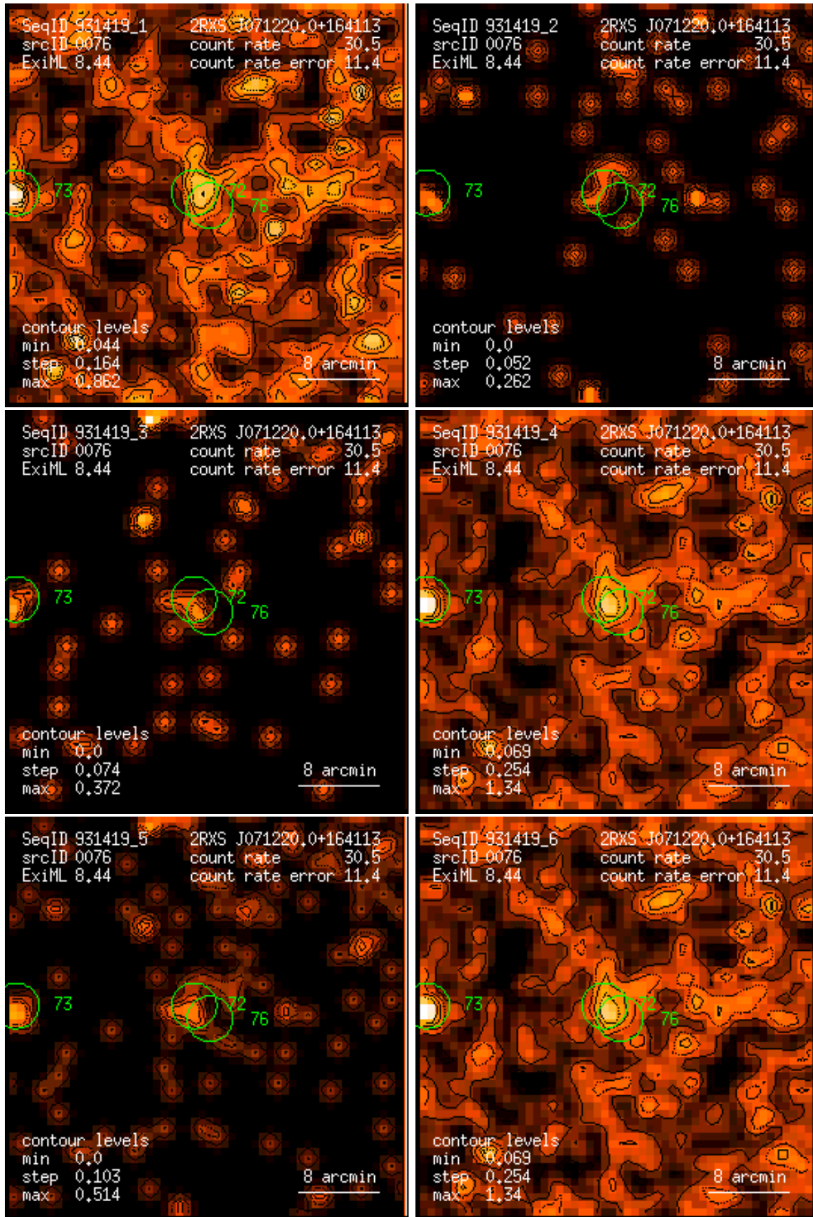
Figure 76: RASS 931419: detection 0076: band rate images, Gaussian filter: (1) PSPC channels 11 – 41, (2) 52 – 90, (3) 91 – 201, (4) 11 – 235, (5) 52 – 201, (6) 11 – 201. Broad band rates in counts/ks. Band rate contour levels in counts/ks/arcmin 2 .
