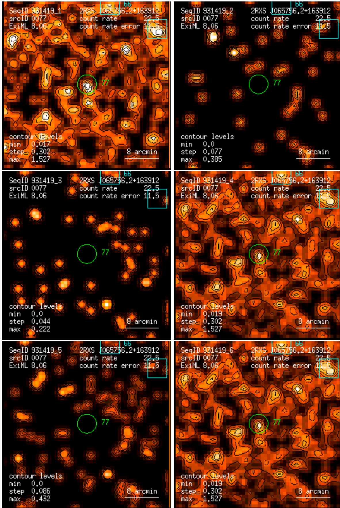
Figure 77: RASS 931419: detection 0077: band rate images, Gaussian filter: (1) PSPC channels 11 – 41, (2) 52 – 90, (3) 91 – 201, (4) 11 – 235, (5) 52 – 201, (6) 11 – 201. Broad band rates in counts/ks. Band rate contour levels in counts/ks/arcmin 2 .
