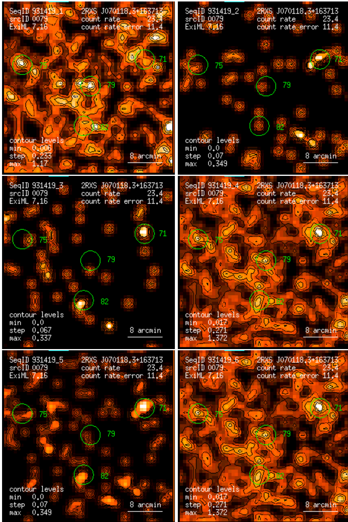
Figure 79: RASS 931419: detection 0079: band rate images, Gaussian filter: (1) PSPC channels 11 – 41, (2) 52 – 90, (3) 91 – 201, (4) 11 – 235, (5) 52 – 201, (6) 11 – 201. Broad band rates in counts/ks. Band rate contour levels in counts/ks/arcmin 2 .
