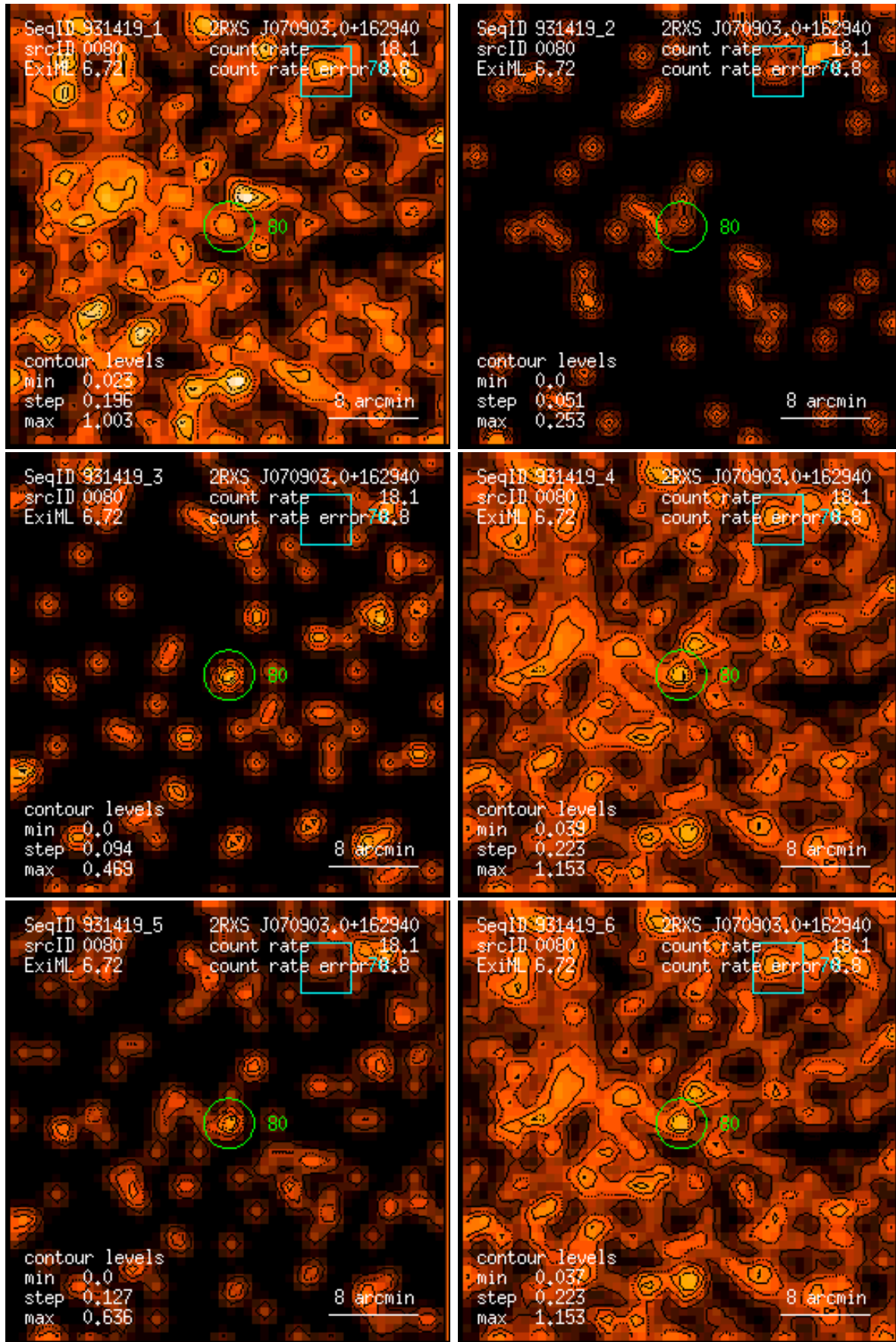
Figure 80: RASS 931419: detection 0080: band rate images, Gaussian filter: (1) PSPC channels 11 – 41, (2) 52 – 90, (3) 91 – 201, (4) 11 – 235, (5) 52 – 201, (6) 11 – 201. Broad band rates in counts/ks. Band rate contour levels in counts/ks/arcmin 2 .
