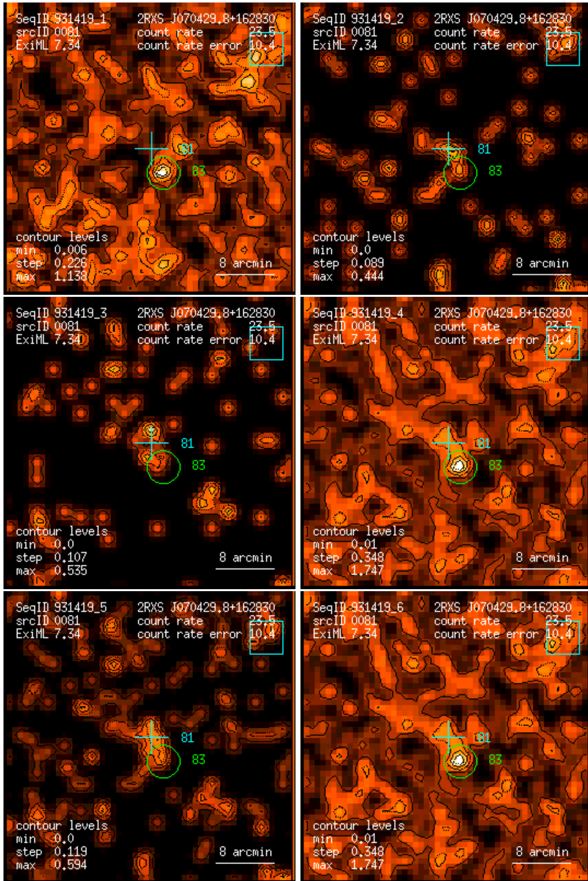
Figure 81: RASS 931419: detection 0081: band rate images, Gaussian filter: (1) PSPC channels 11 – 41, (2) 52 – 90, (3) 91 – 201, (4) 11 – 235, (5) 52 – 201, (6) 11 – 201. Broad band rates in counts/ks. Band rate contour levels in counts/ks/arcmin 2 .
