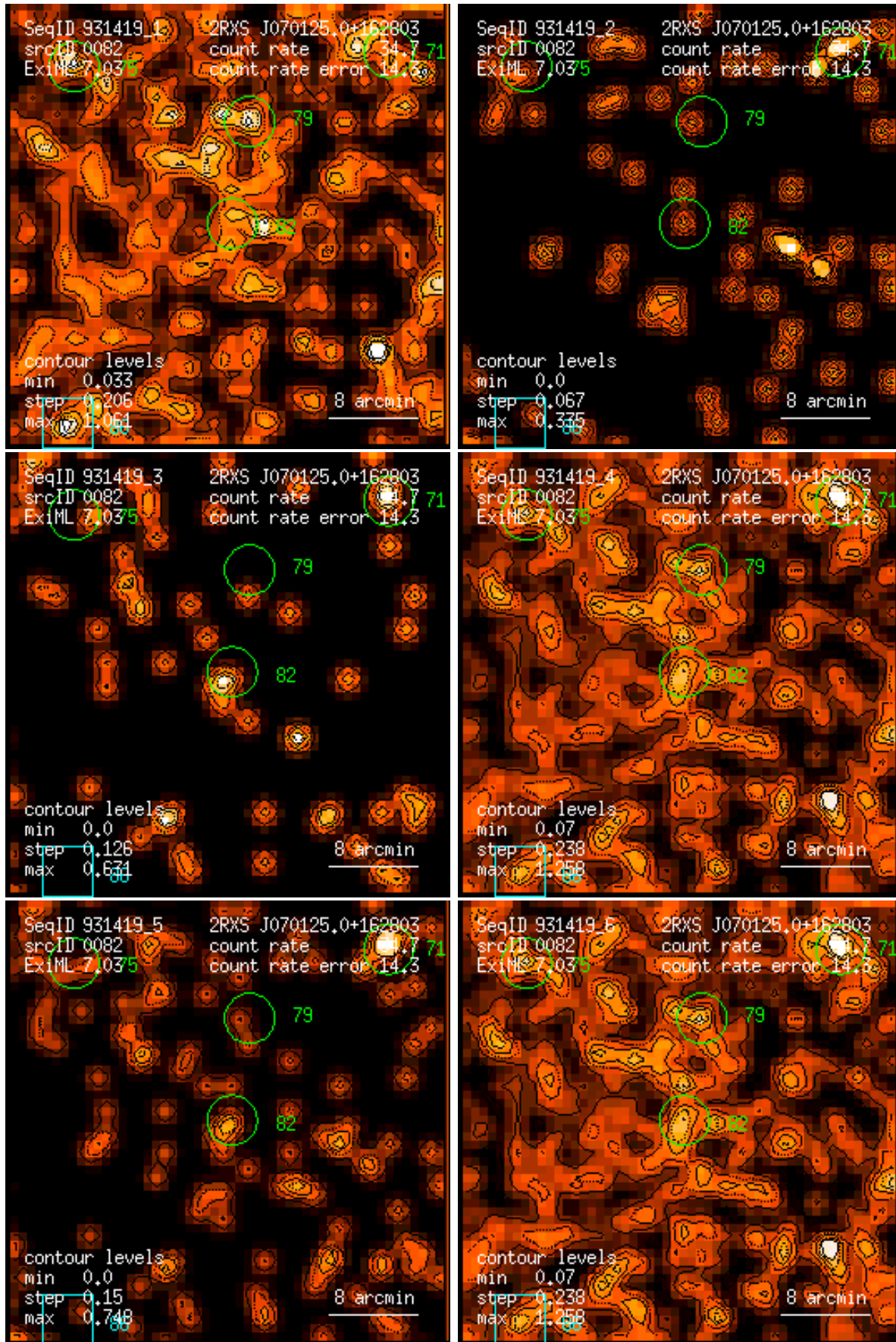
Figure 82: RASS 931419: detection 0082: band rate images, Gaussian filter: (1) PSPC channels 11 – 41, (2) 52 – 90, (3) 91 – 201, (4) 11 – 235, (5) 52 – 201, (6) 11 – 201. Broad band rates in counts/ks. Band rate contour levels in counts/ks/arcmin 2 .
