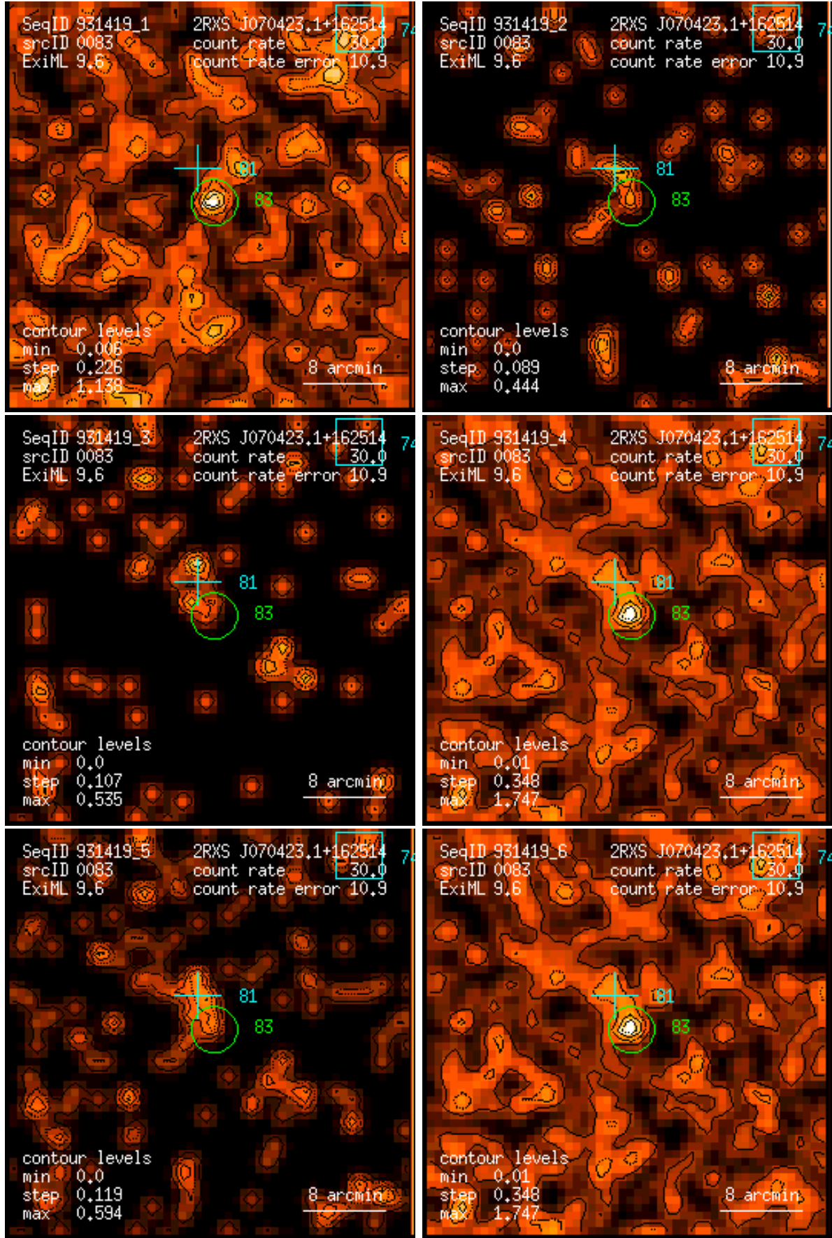
Figure 83: RASS 931419: detection 0083: band rate images, Gaussian filter: (1) PSPC channels 11 – 41, (2) 52 – 90, (3) 91 – 201, (4) 11 – 235, (5) 52 – 201, (6) 11 – 201. Broad band rates in counts/ks. Band rate contour levels in counts/ks/arcmin 2 .
