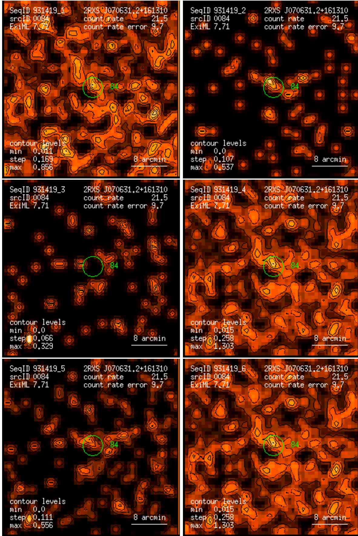
Figure 84: RASS 931419: detection 0084: band rate images, Gaussian filter: (1) PSPC channels 11 – 41, (2) 52 – 90, (3) 91 – 201, (4) 11 – 235, (5) 52 – 201, (6) 11 – 201. Broad band rates in counts/ks. Band rate contour levels in counts/ks/arcmin 2 .
