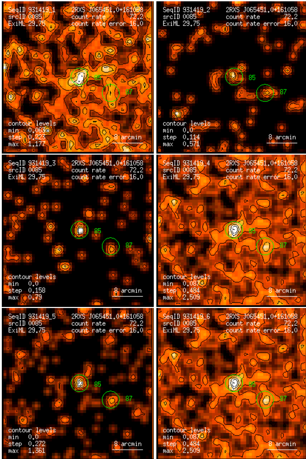
Figure 85: RASS 931419: detection 0085: band rate images, Gaussian filter: (1) PSPC channels 11 – 41, (2) 52 – 90, (3) 91 – 201, (4) 11 – 235, (5) 52 – 201, (6) 11 – 201. Broad band rates in counts/ks. Band rate contour levels in counts/ks/arcmin 2 .
