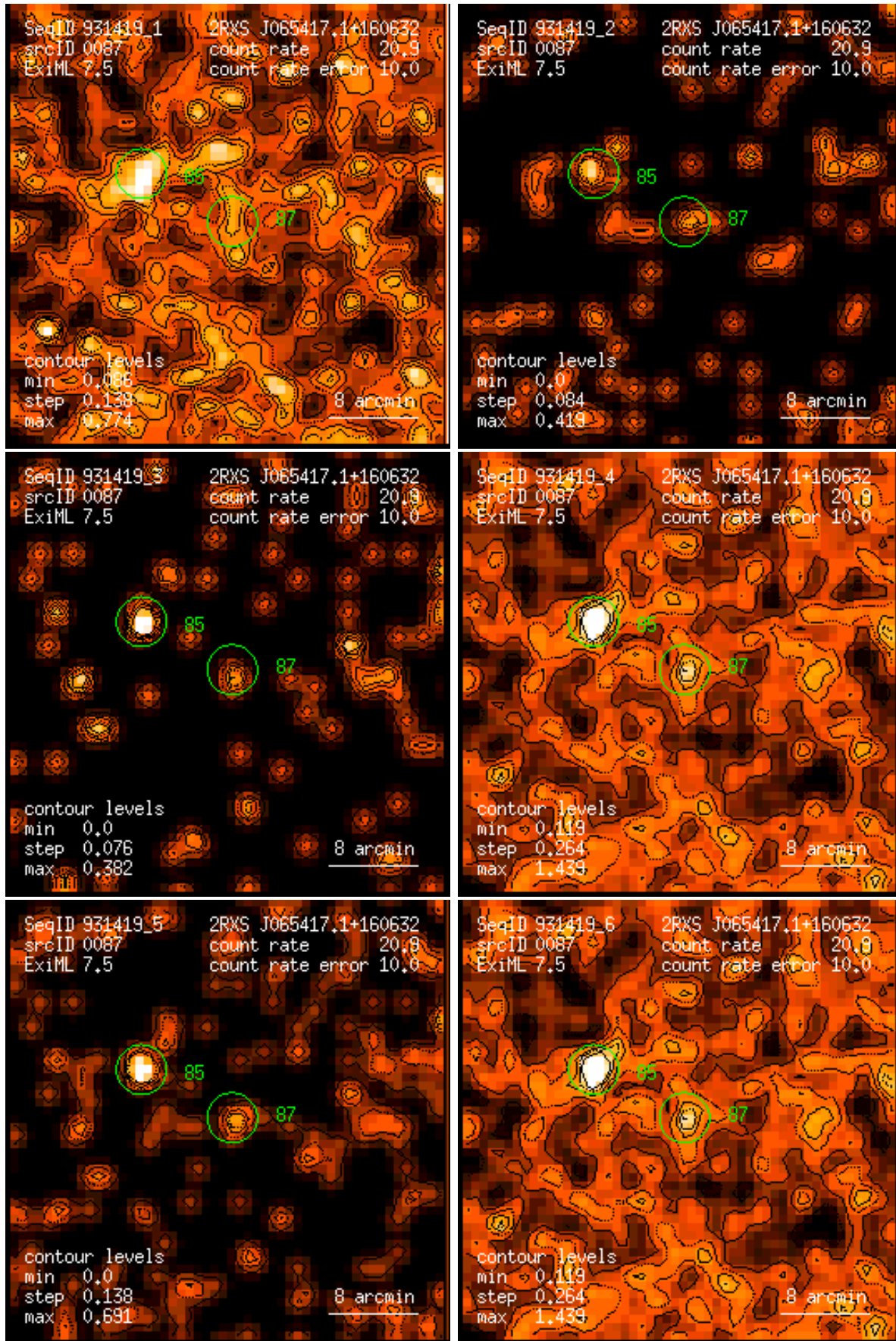
Figure 87: RASS 931419: detection 0087: band rate images, Gaussian filter: (1) PSPC channels 11 – 41, (2) 52 – 90, (3) 91 – 201, (4) 11 – 235, (5) 52 – 201, (6) 11 – 201. Broad band rates in counts/ks. Band rate contour levels in counts/ks/arcmin 2 .
