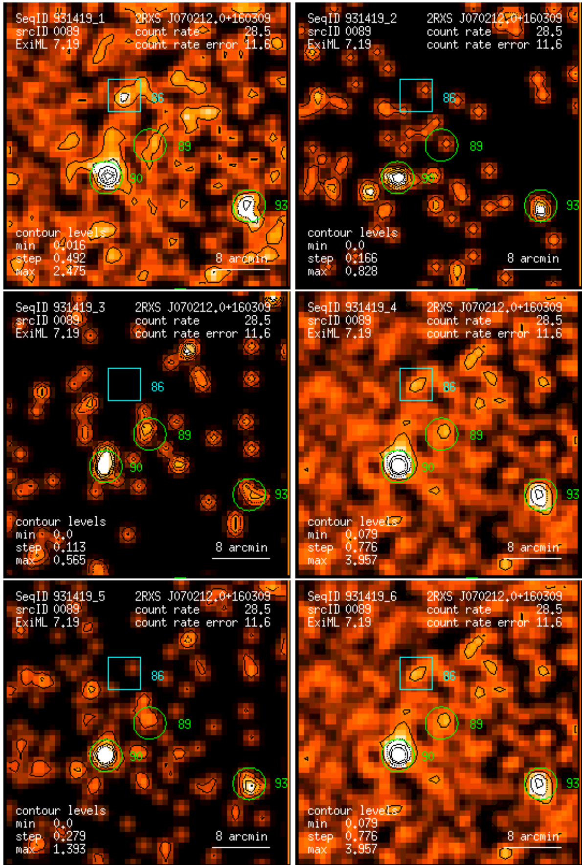
Figure 89: RASS 931419: detection 0089: band rate images, Gaussian filter: (1) PSPC channels 11 – 41, (2) 52 – 90, (3) 91 – 201, (4) 11 – 235, (5) 52 – 201, (6) 11 – 201. Broad band rates in counts/ks. Band rate contour levels in counts/ks/arcmin 2 .
