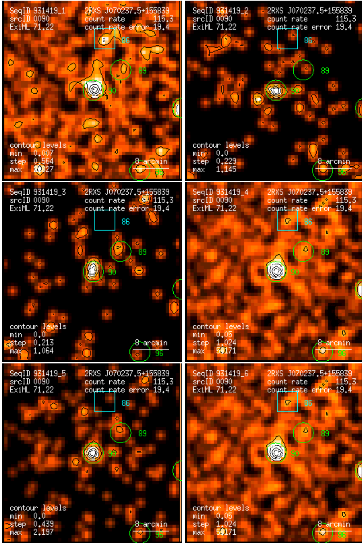
Figure 90: RASS 931419: detection 0090: band rate images, Gaussian filter: (1) PSPC channels 11 – 41, (2) 52 – 90, (3) 91 – 201, (4) 11 – 235, (5) 52 – 201, (6) 11 – 201. Broad band rates in counts/ks. Band rate contour levels in counts/ks/arcmin 2 .
