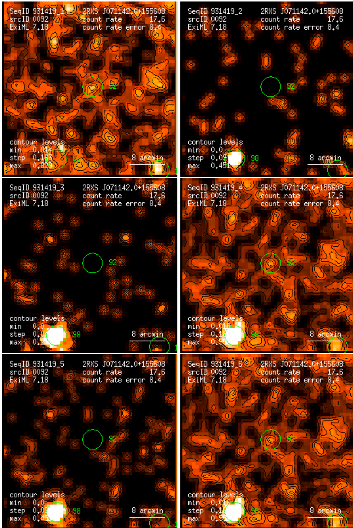
Figure 92: RASS 931419: detection 0092: band rate images, Gaussian filter: (1) PSPC channels 11 – 41, (2) 52 – 90, (3) 91 – 201, (4) 11 – 235, (5) 52 – 201, (6) 11 – 201. Broad band rates in counts/ks. Band rate contour levels in counts/ks/arcmin 2 .
