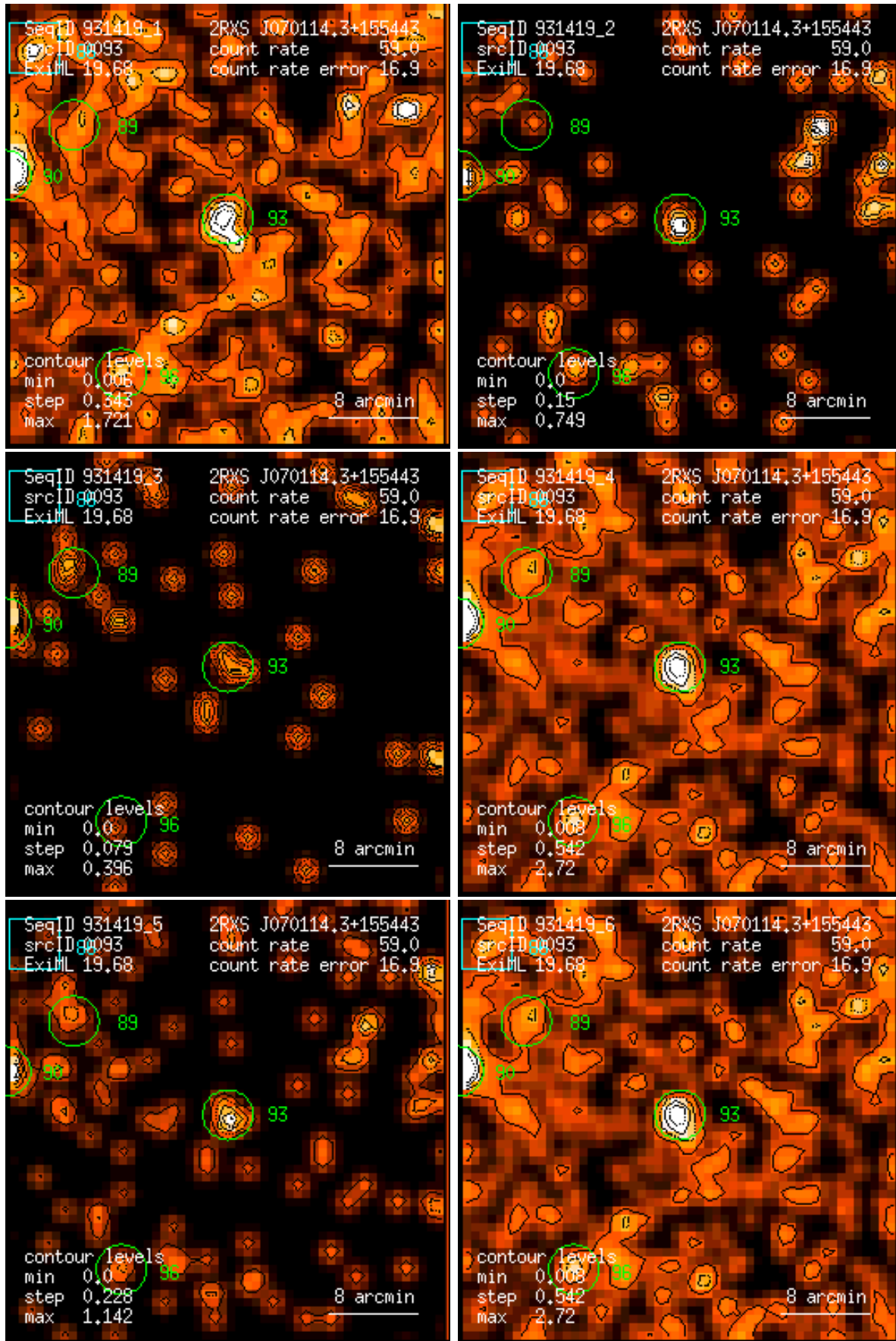
Figure 93: RASS 931419: detection 0093: band rate images, Gaussian filter: (1) PSPC channels 11 – 41, (2) 52 – 90, (3) 91 – 201, (4) 11 – 235, (5) 52 – 201, (6) 11 – 201. Broad band rates in counts/ks. Band rate contour levels in counts/ks/arcmin 2 .
