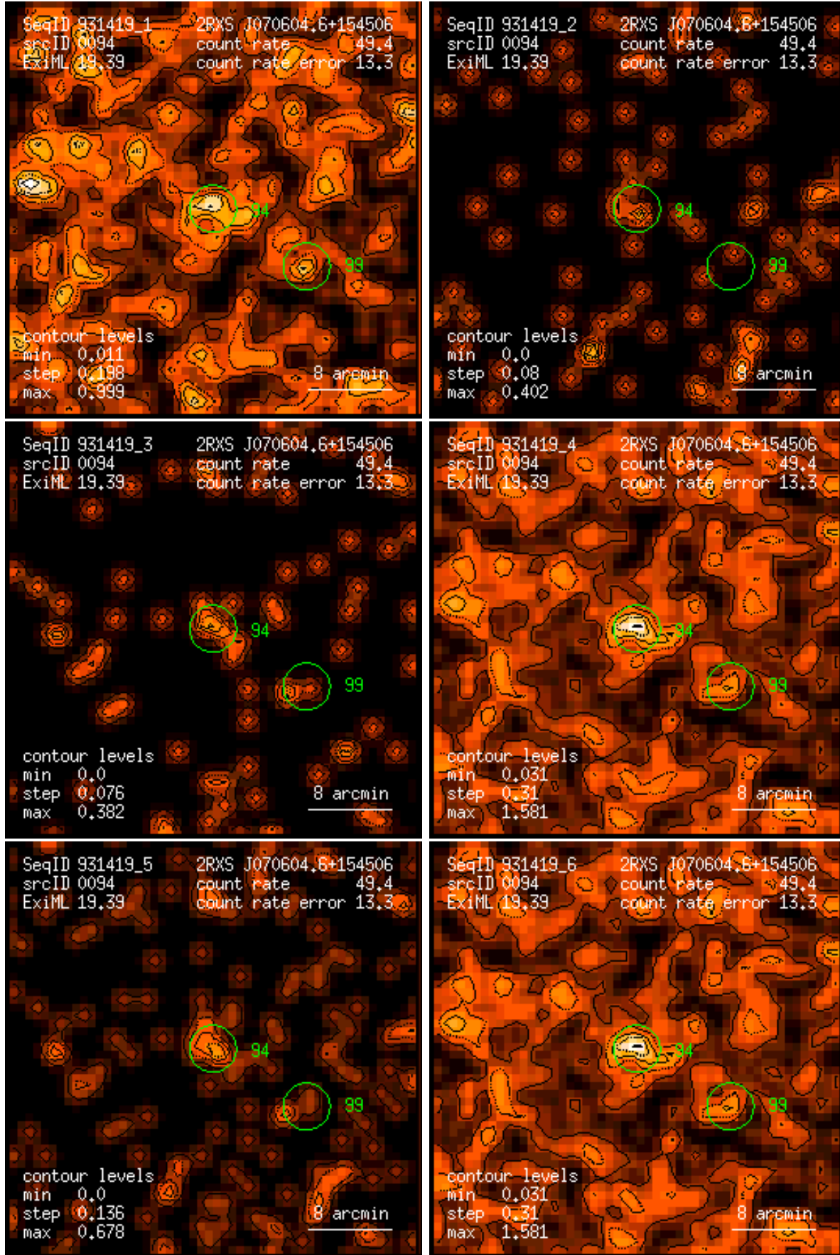
Figure 94: RASS 931419: detection 0094: band rate images, Gaussian filter: (1) PSPC channels 11 – 41, (2) 52 – 90, (3) 91 – 201, (4) 11 – 235, (5) 52 – 201, (6) 11 – 201. Broad band rates in counts/ks. Band rate contour levels in counts/ks/arcmin 2 .
