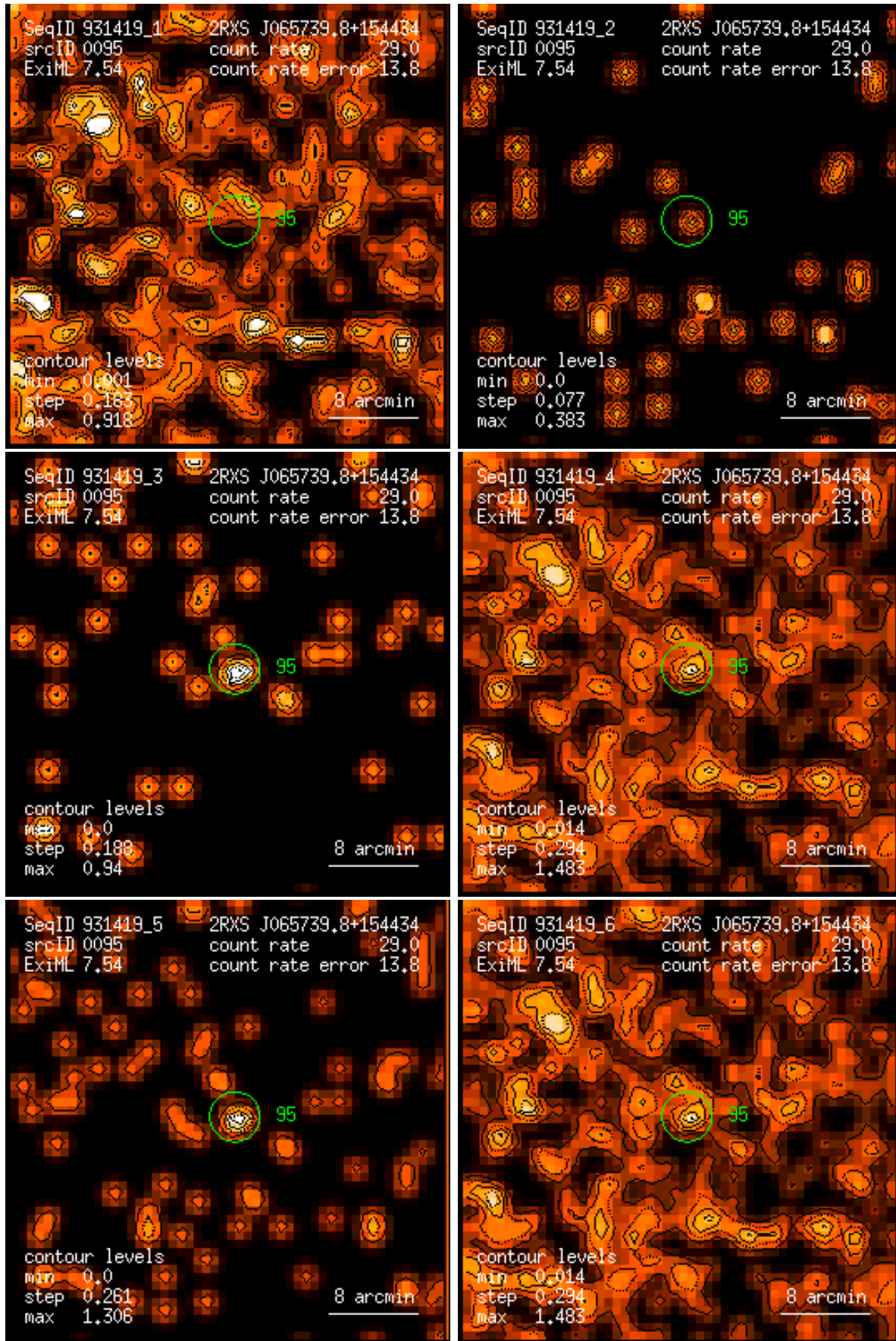
Figure 95: RASS 931419: detection 0095: band rate images, Gaussian filter: (1) PSPC channels 11 – 41, (2) 52 – 90, (3) 91 – 201, (4) 11 – 235, (5) 52 – 201, (6) 11 – 201. Broad band rates in counts/ks. Band rate contour levels in counts/ks/arcmin 2 .
