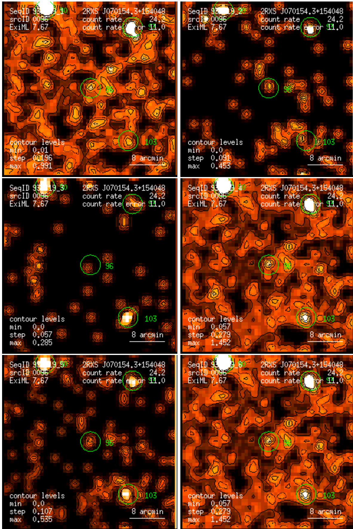
Figure 96: RASS 931419: detection 0096: band rate images, Gaussian filter: (1) PSPC channels 11 – 41, (2) 52 – 90, (3) 91 – 201, (4) 11 – 235, (5) 52 – 201, (6) 11 – 201. Broad band rates in counts/ks. Band rate contour levels in counts/ks/arcmin 2 .
