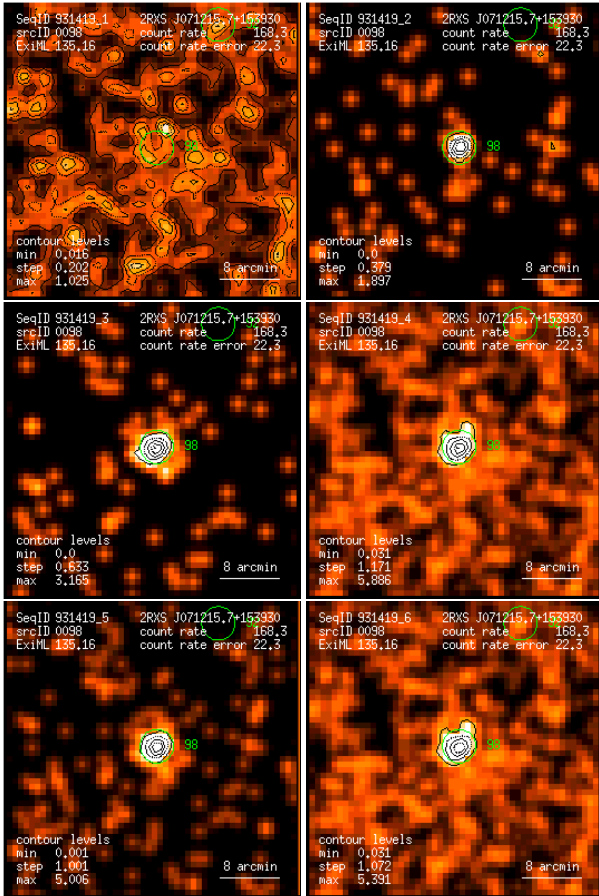
Figure 98: RASS 931419: detection 0098: band rate images, Gaussian filter: (1) PSPC channels 11 – 41, (2) 52 – 90, (3) 91 – 201, (4) 11 – 235, (5) 52 – 201, (6) 11 – 201. Broad band rates in counts/ks. Band rate contour levels in counts/ks/arcmin 2 .
