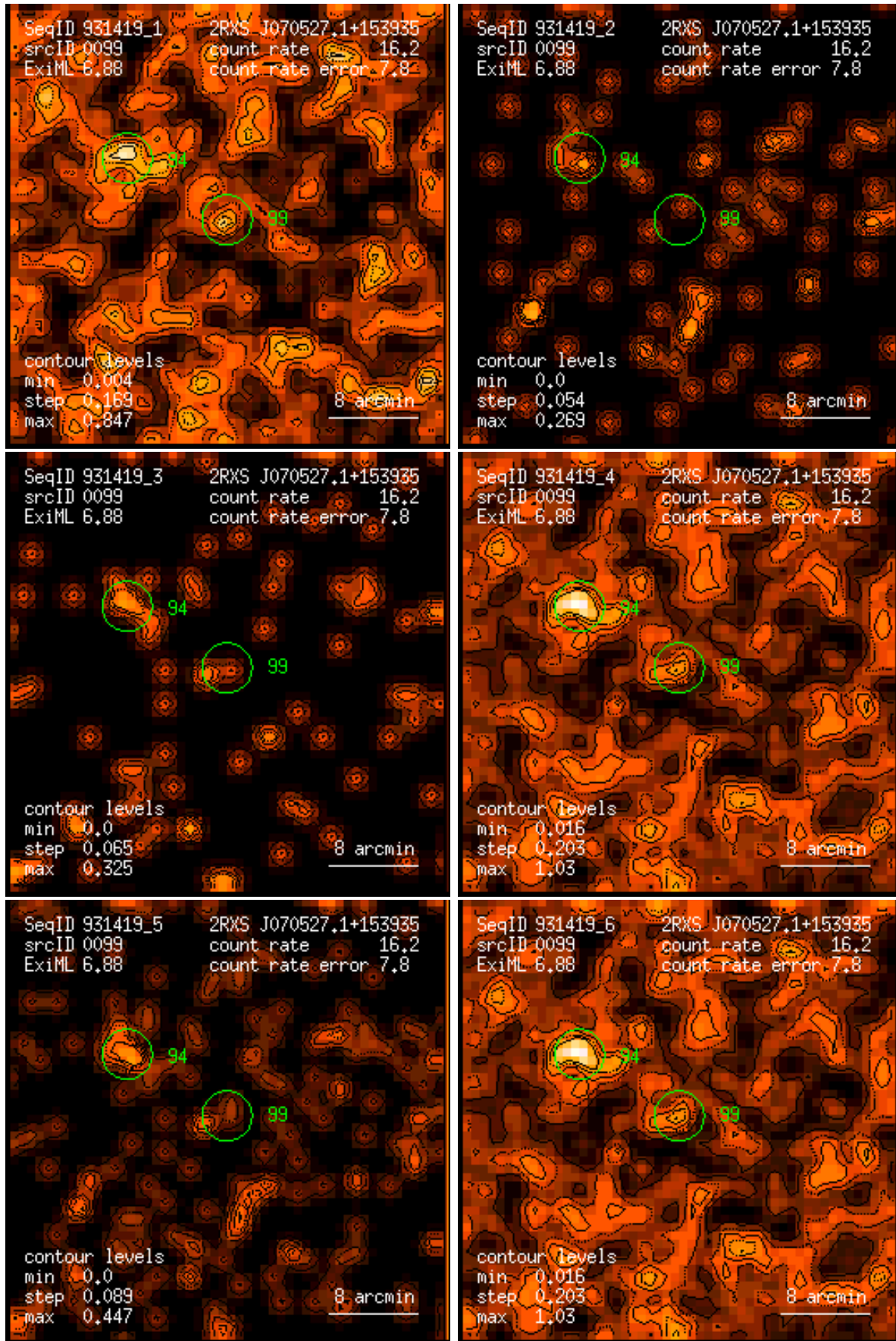
Figure 99: RASS 931419: detection 0099: band rate images, Gaussian filter: (1) PSPC channels 11 – 41, (2) 52 – 90, (3) 91 – 201, (4) 11 – 235, (5) 52 – 201, (6) 11 – 201. Broad band rates in counts/ks. Band rate contour levels in counts/ks/arcmin 2 .
