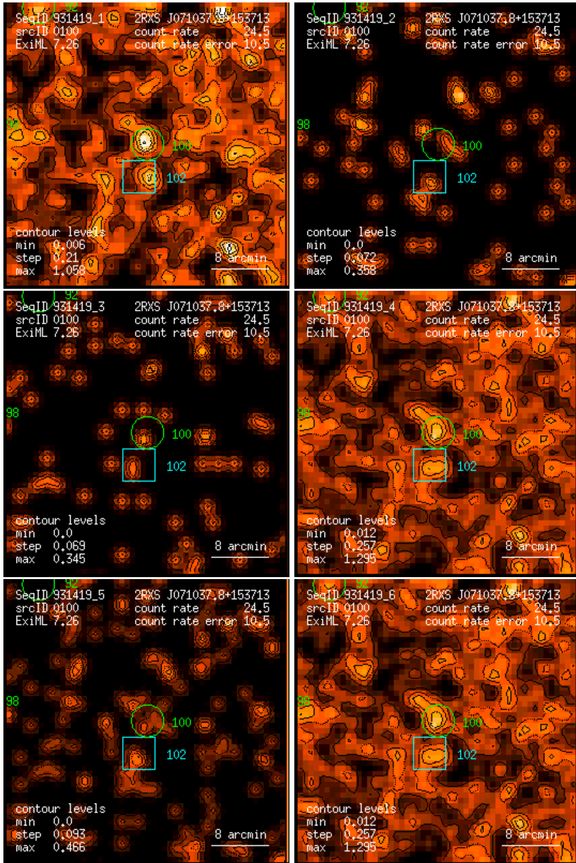
Figure 100: RASS 931419: detection 0100: band rate images, Gaussian filter: (1) PSPC channels 11 – 41, (2) 52 – 90, (3) 91 – 201, (4) 11 – 235, (5) 52 – 201, (6) 11 – 201. Broad band rates in counts/ks. Band rate contour levels in counts/ks/arcmin 2 .
