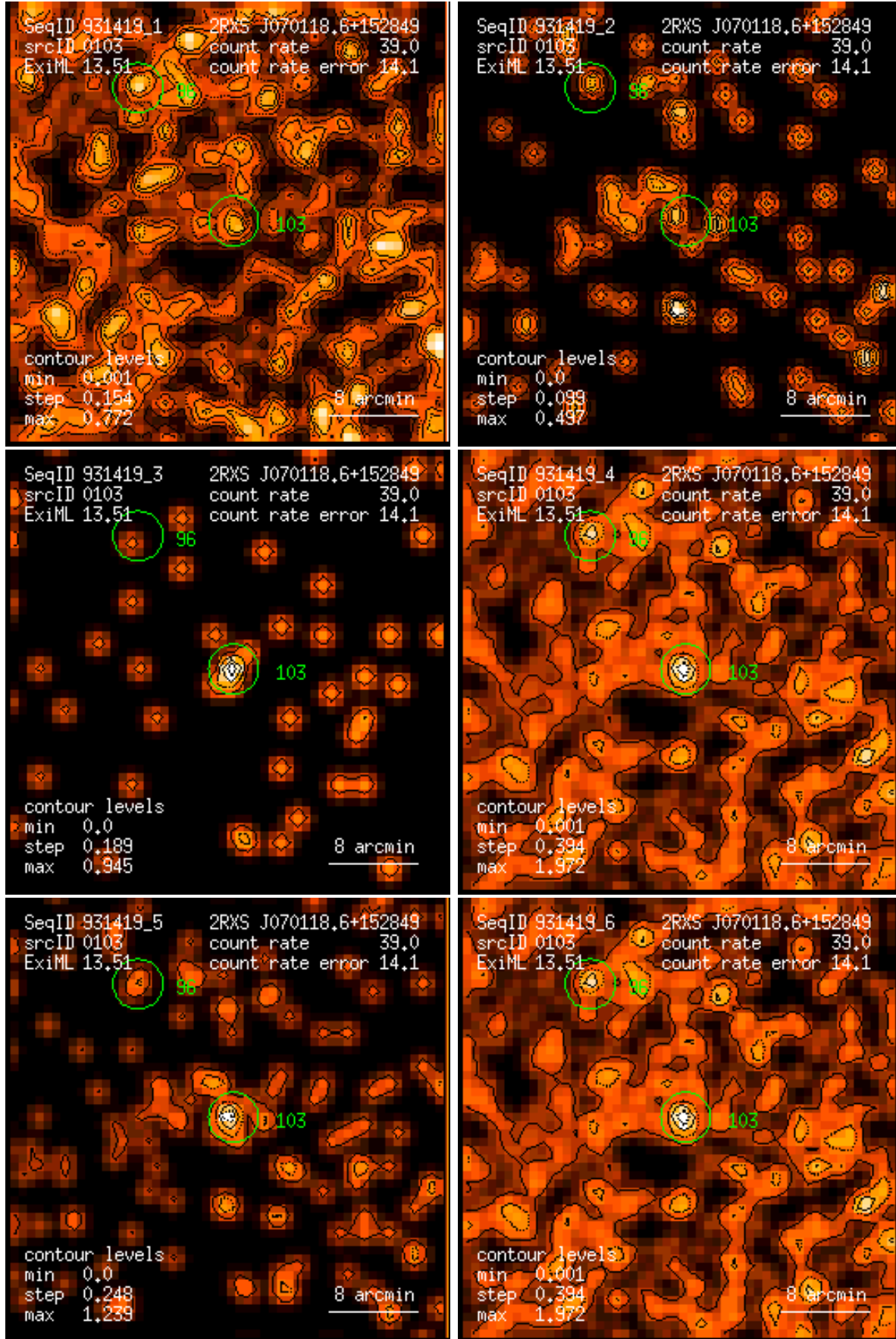
Figure 103: RASS 931419: detection 0103: band rate images, Gaussian filter: (1) PSPC channels 11 – 41, (2) 52 – 90, (3) 91 – 201, (4) 11 – 235, (5) 52 – 201, (6) 11 – 201. Broad band rates in counts/ks. Band rate contour levels in counts/ks/arcmin 2 .
