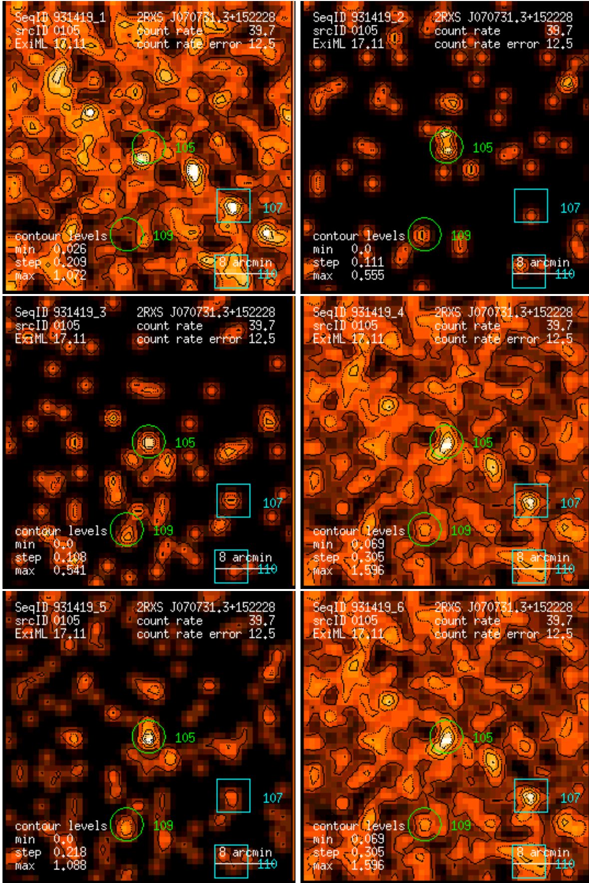
Figure 105: RASS 931419: detection 0105: band rate images, Gaussian filter: (1) PSPC channels 11 – 41, (2) 52 – 90, (3) 91 – 201, (4) 11 – 235, (5) 52 – 201, (6) 11 – 201. Broad band rates in counts/ks. Band rate contour levels in counts/ks/arcmin 2 .
