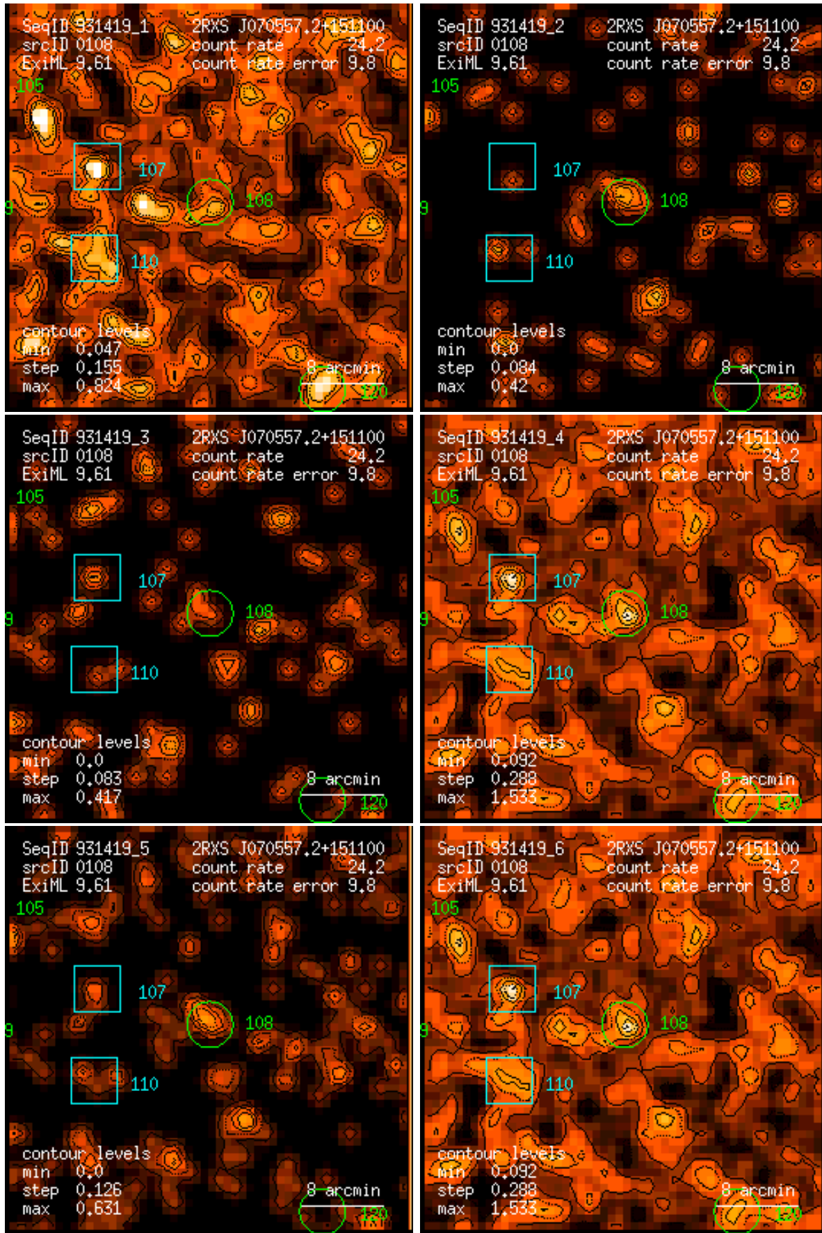
Figure 108: RASS 931419: detection 0108: band rate images, Gaussian filter: (1) PSPC channels 11 – 41, (2) 52 – 90, (3) 91 – 201, (4) 11 – 235, (5) 52 – 201, (6) 11 – 201. Broad band rates in counts/ks. Band rate contour levels in counts/ks/arcmin 2 .
