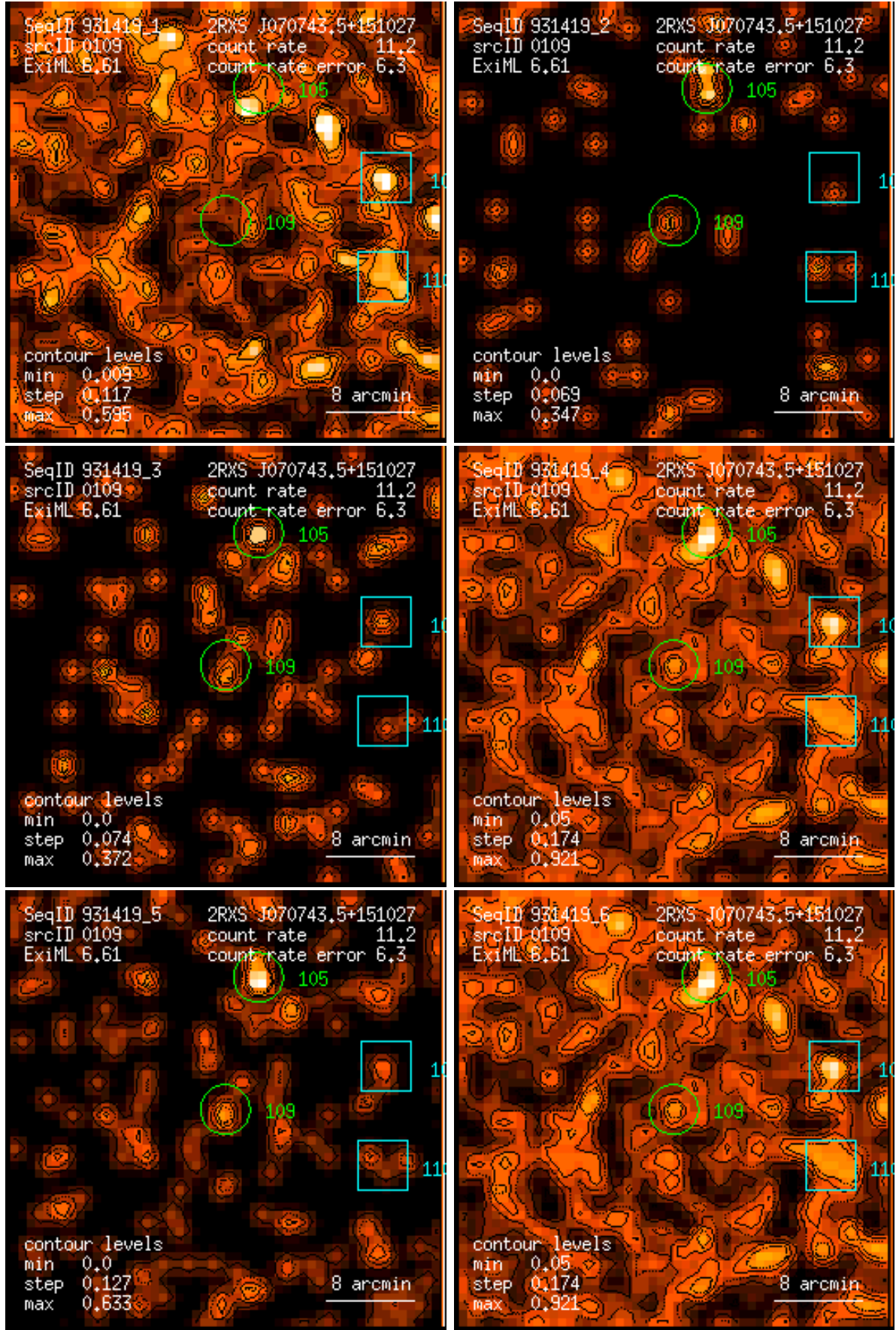
Figure 109: RASS 931419: detection 0109: band rate images, Gaussian filter: (1) PSPC channels 11 – 41, (2) 52 – 90, (3) 91 – 201, (4) 11 – 235, (5) 52 – 201, (6) 11 – 201. Broad band rates in counts/ks. Band rate contour levels in counts/ks/arcmin 2 .
