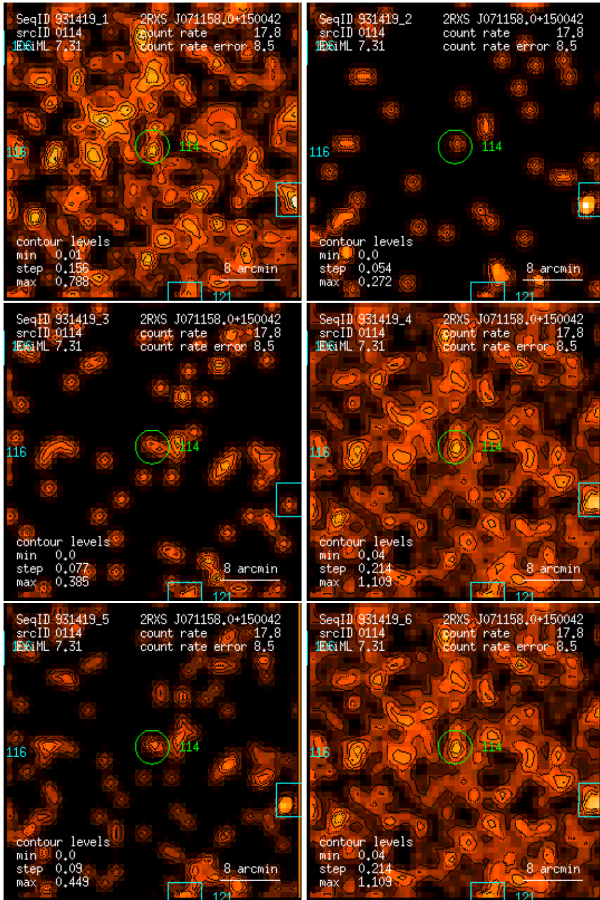
Figure 114: RASS 931419: detection 0114: band rate images, Gaussian filter: (1) PSPC channels 11 – 41, (2) 52 – 90, (3) 91 – 201, (4) 11 – 235, (5) 52 – 201, (6) 11 – 201. Broad band rates in counts/ks. Band rate contour levels in counts/ks/arcmin 2 .
