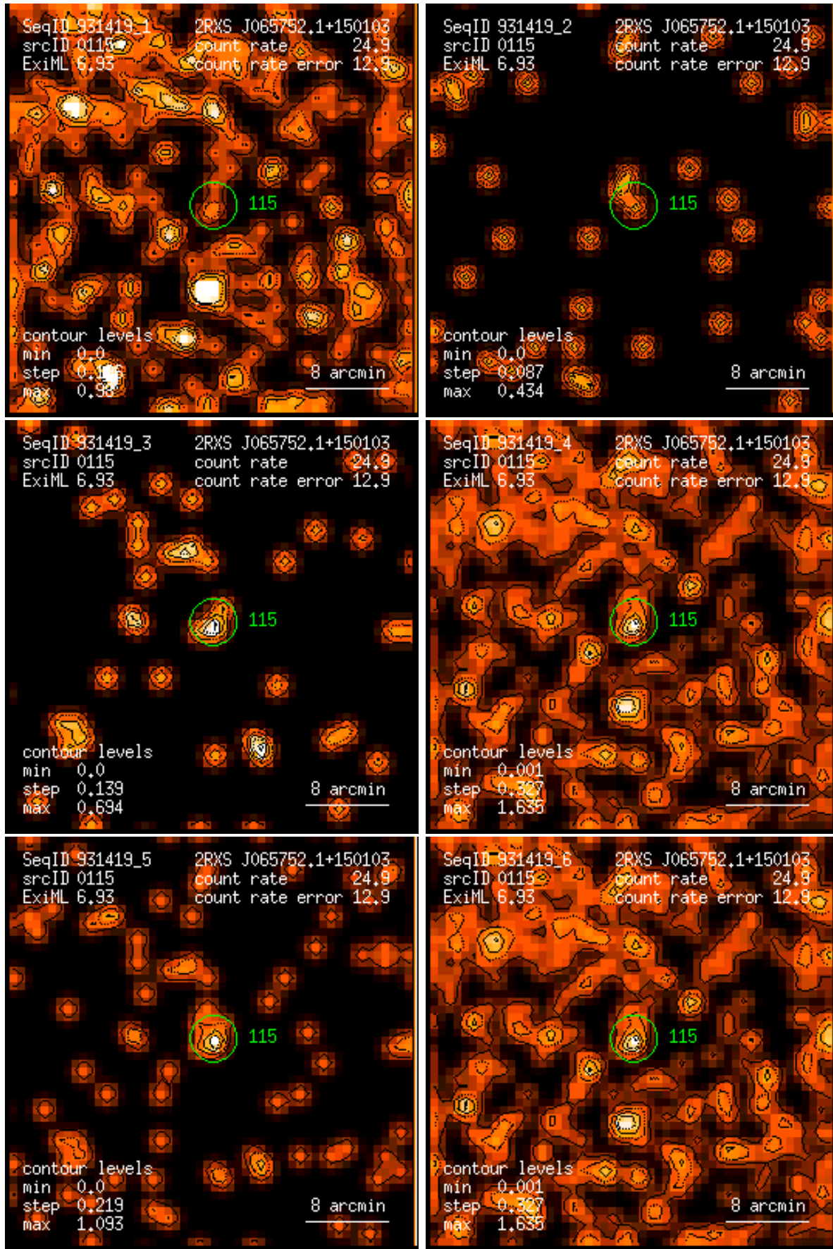
Figure 115: RASS 931419: detection 0115: band rate images, Gaussian filter: (1) PSPC channels 11 – 41, (2) 52 – 90, (3) 91 – 201, (4) 11 – 235, (5) 52 – 201, (6) 11 – 201. Broad band rates in counts/ks. Band rate contour levels in counts/ks/arcmin 2 .
