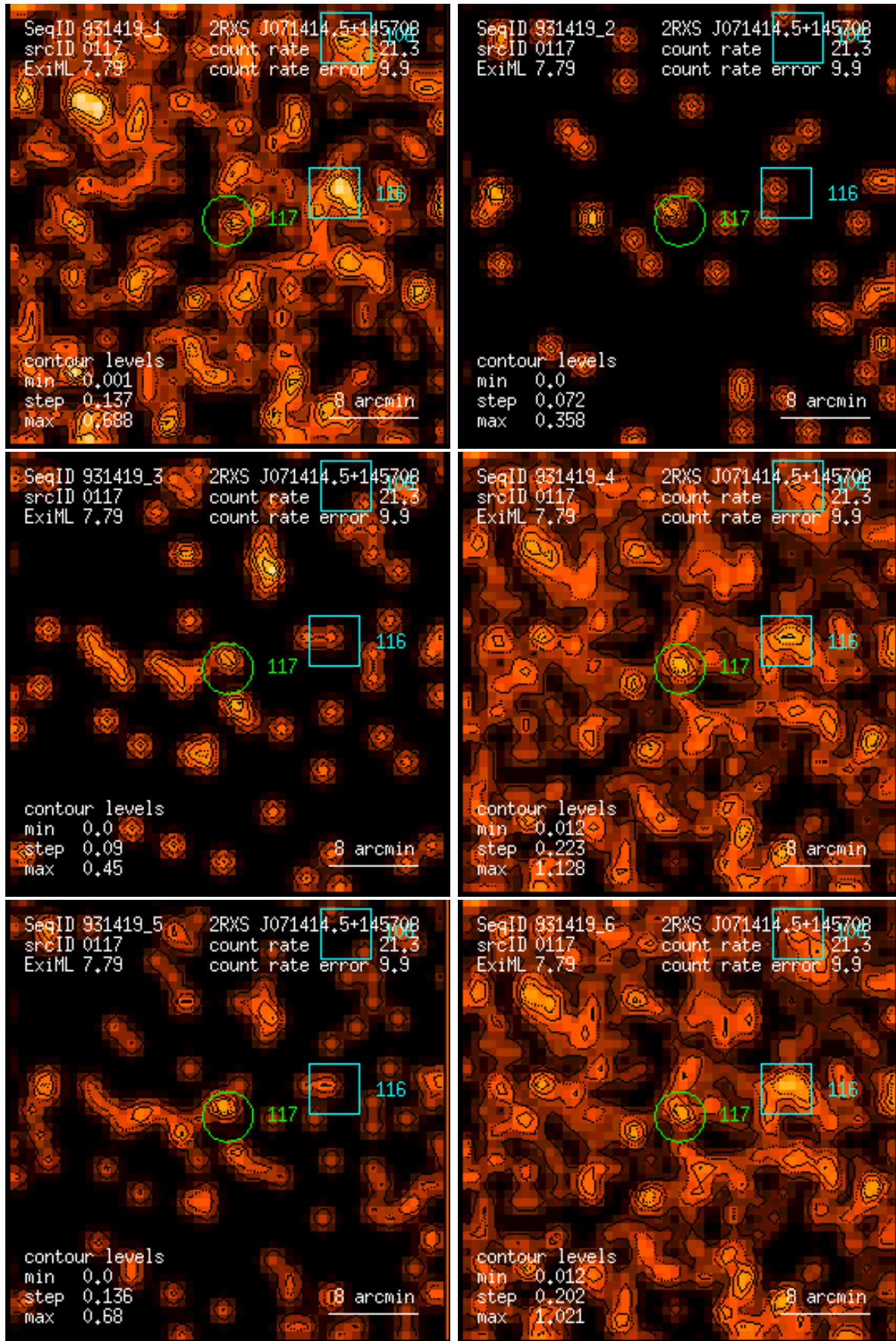
Figure 117: RASS 931419: detection 0117: band rate images, Gaussian filter: (1) PSPC channels 11 – 41, (2) 52 – 90, (3) 91 – 201, (4) 11 – 235, (5) 52 – 201, (6) 11 – 201. Broad band rates in counts/ks. Band rate contour levels in counts/ks/arcmin 2 .
