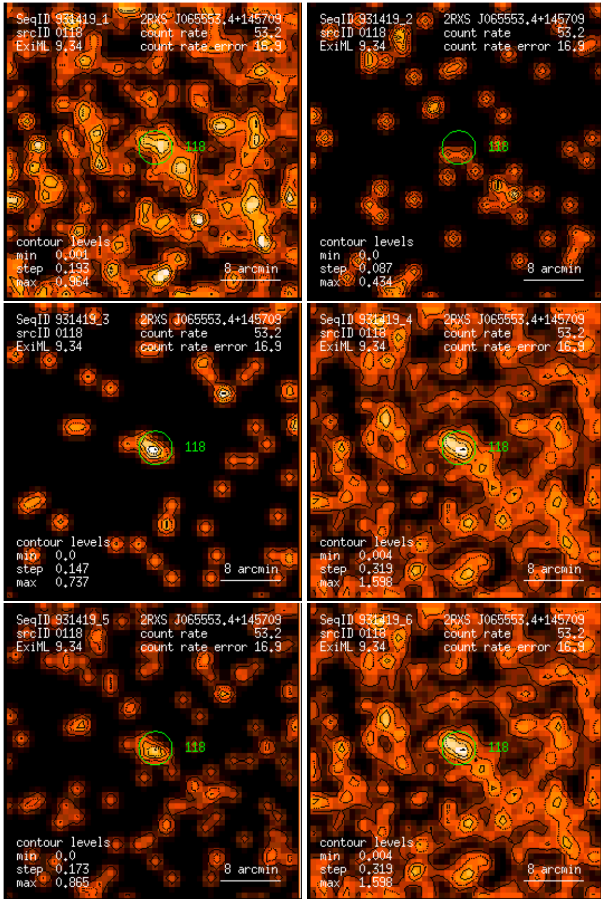
Figure 118: RASS 931419: detection 0118: band rate images, Gaussian filter: (1) PSPC channels 11 – 41, (2) 52 – 90, (3) 91 – 201, (4) 11 – 235, (5) 52 – 201, (6) 11 – 201. Broad band rates in counts/ks. Band rate contour levels in counts/ks/arcmin 2 .
