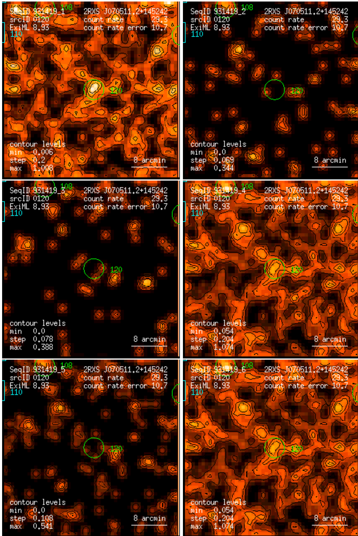
Figure 120: RASS 931419: detection 0120: band rate images, Gaussian filter: (1) PSPC channels 11 – 41, (2) 52 – 90, (3) 91 – 201, (4) 11 – 235, (5) 52 – 201, (6) 11 – 201. Broad band rates in counts/ks. Band rate contour levels in counts/ks/arcmin 2 .
