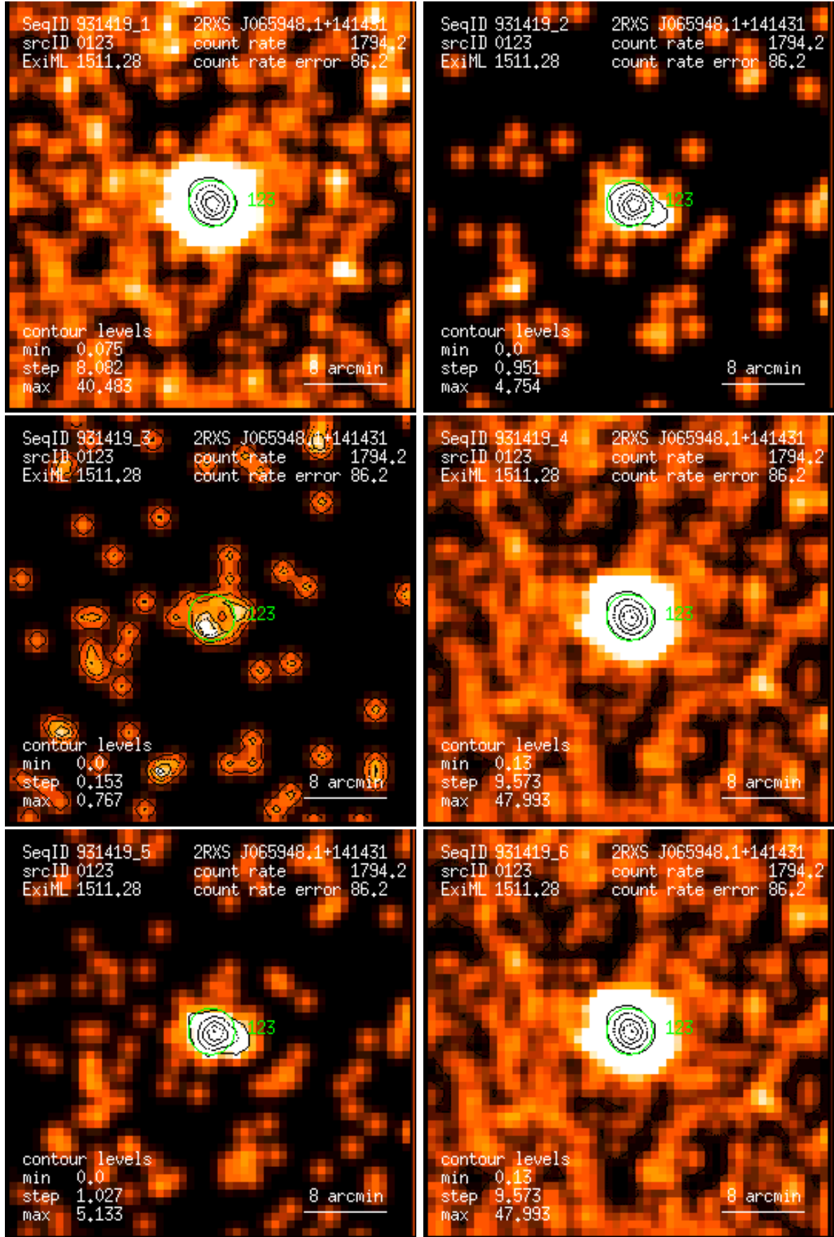
Figure 123: RASS 931419: detection 0123: band rate images, Gaussian filter: (1) PSPC channels 11 – 41, (2) 52 – 90, (3) 91 – 201, (4) 11 – 235, (5) 52 – 201, (6) 11 – 201. Broad band rates in counts/ks. Band rate contour levels in counts/ks/arcmin 2 .
